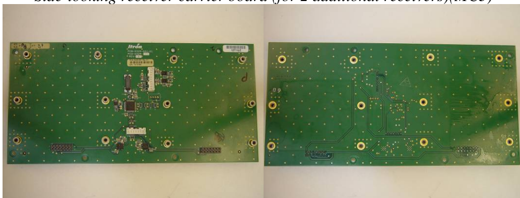
Side-looking receiver carrier board (for 2 additional receivers)(MC3)
