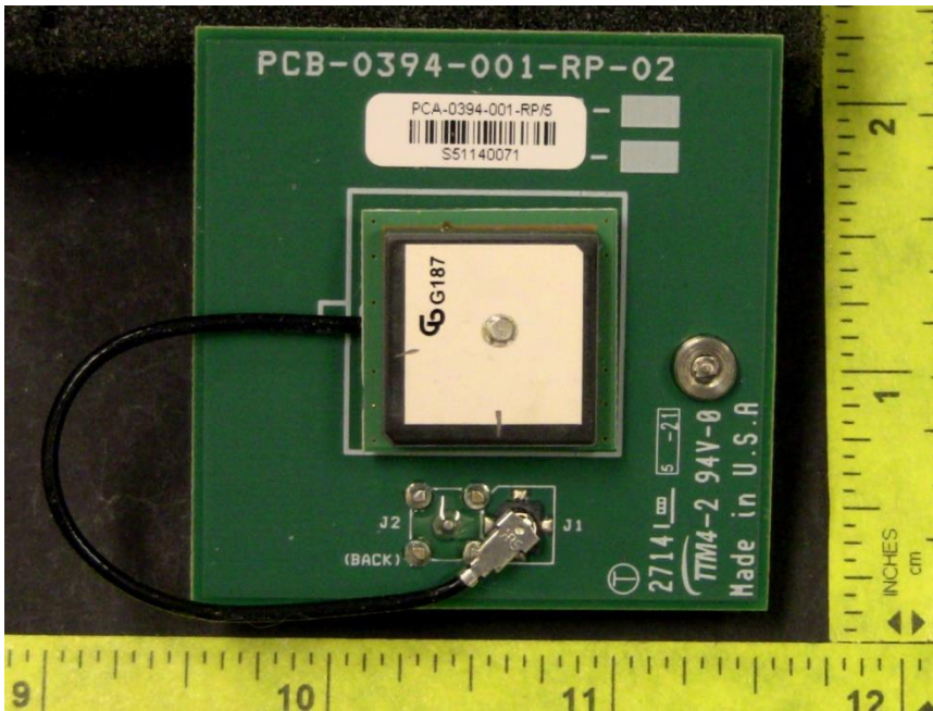
Detail of GPS Antenna Board front.
