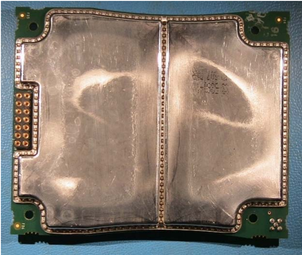
BCR 900MHz – radio – bottom w/shield
