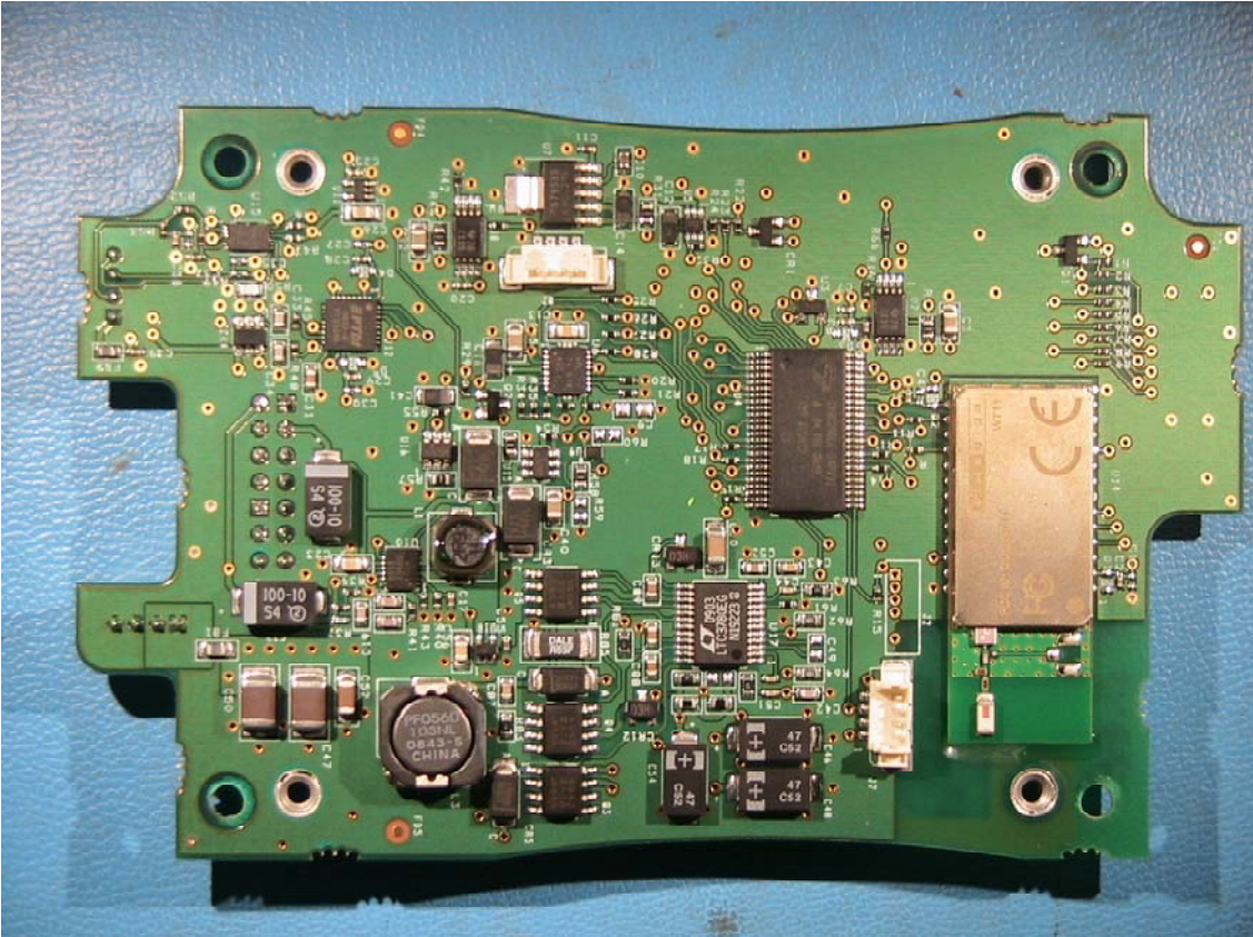
BCR 900MHz - Communications/Carrier – bottom
