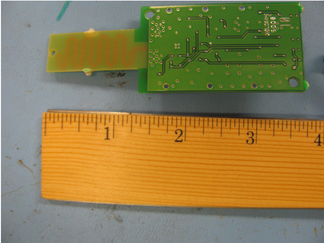
60W internal photos.
