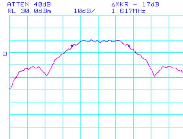
CENTER 2.440000GHz SPAN 5.000MHz *RBW 100kHz *VBW 300kHz SWP 50.0ms Figure 2: 6dB Bandwidth Measurement: f=2440MHz
