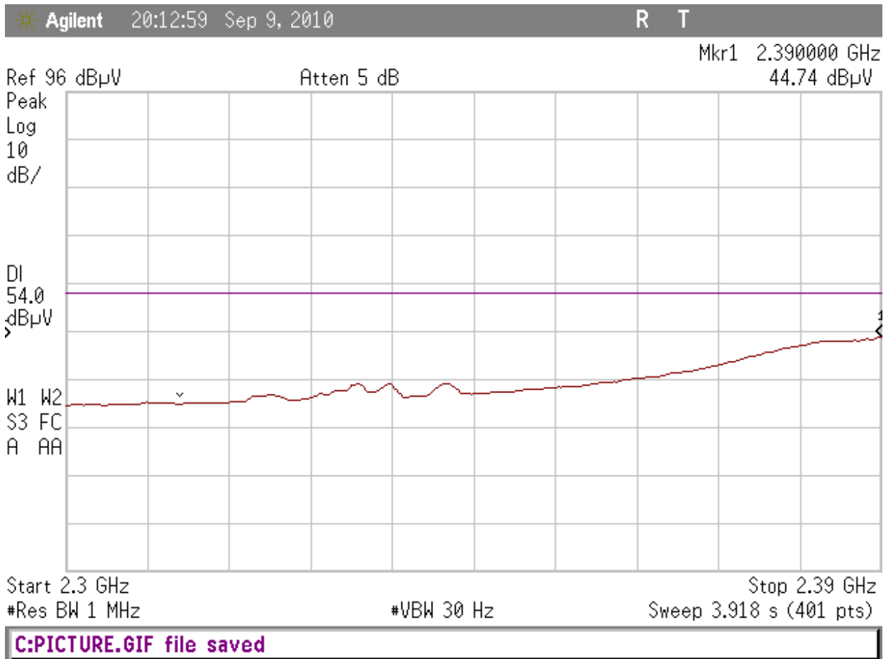
Figure 22: Average Vertical Radiated Band Edge (2405MHz Fundamental)
