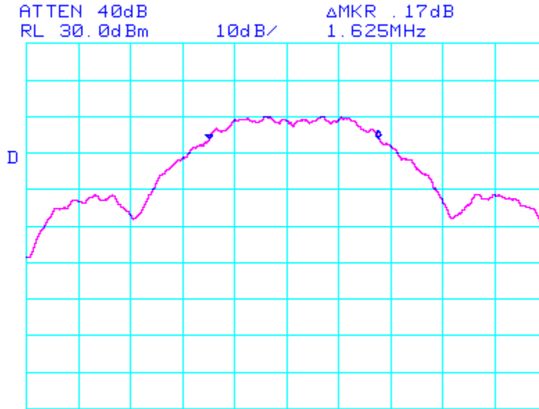
CENTER 2.405000GHz SPAN 5.000MHz *RBW 100kHz *VBW 300kHz SWP 50.0ms Figure 1: 6dB Bandwidth Measurement: f=2405MHz
