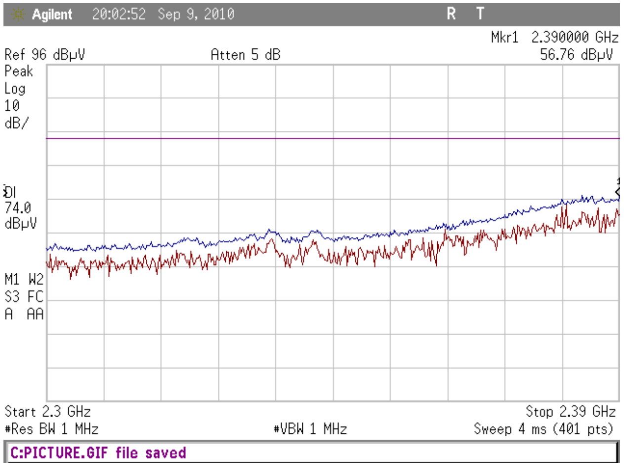
Figure 21: Peak Vertical Radiated Band Edge (2405MHz Fundamental)
