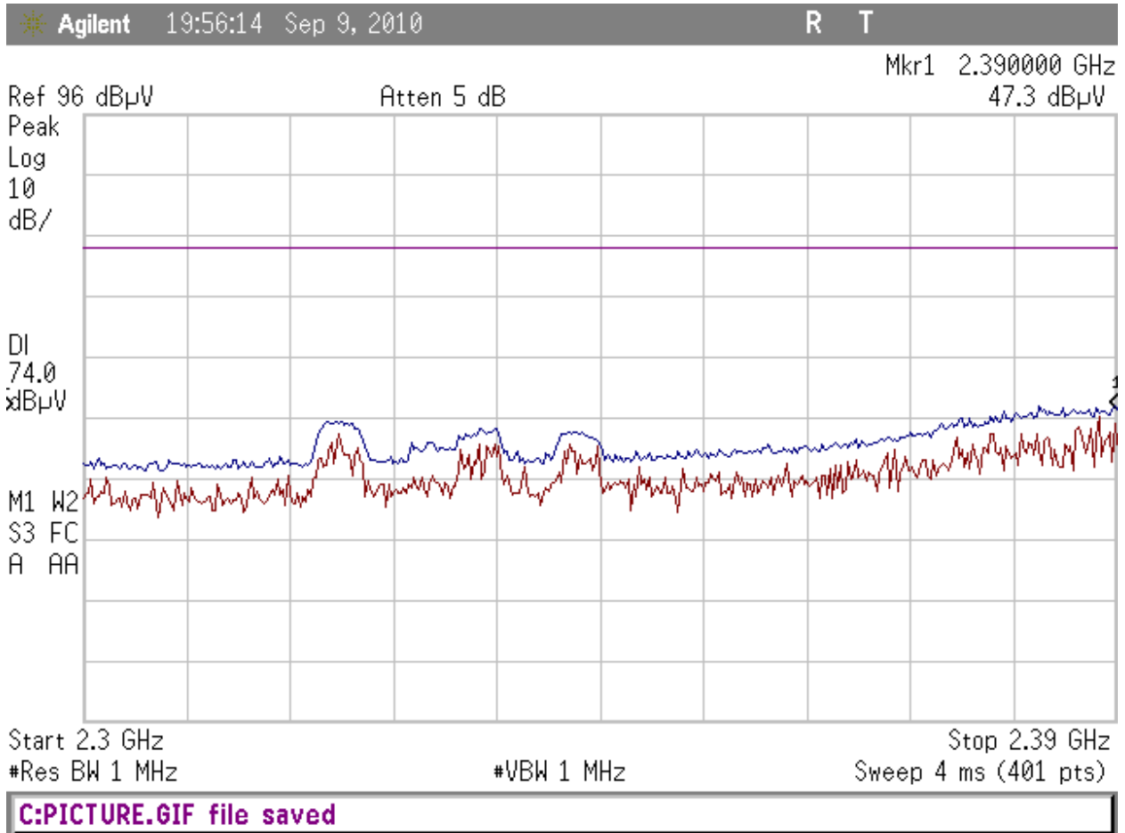
Figure 19: Peak Horizontal Radiated Band Edge (2405MHz Fundamental)
