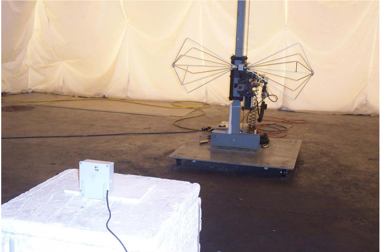
Figure 6: Test Setup for Radiated Spurious measurements between 30MHz and 300MHz using Biconical antenna shown here in horizontal orientation and Remote in foreground
