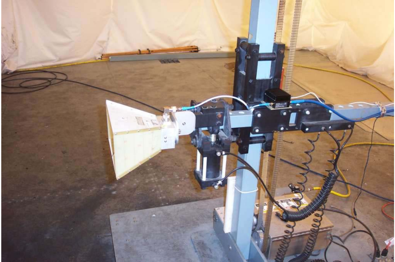
Figure 16: Test setup for TX radiated spurious emissions between 1 and 3GHz (Vertical polarity shown)
