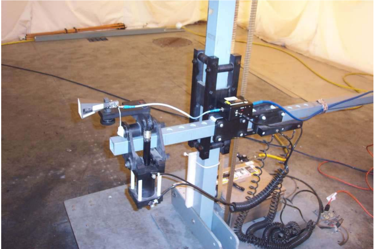
Figure 22: Test setup for radiated spurious emissions above 18GHz (horizontal polarity shown)
