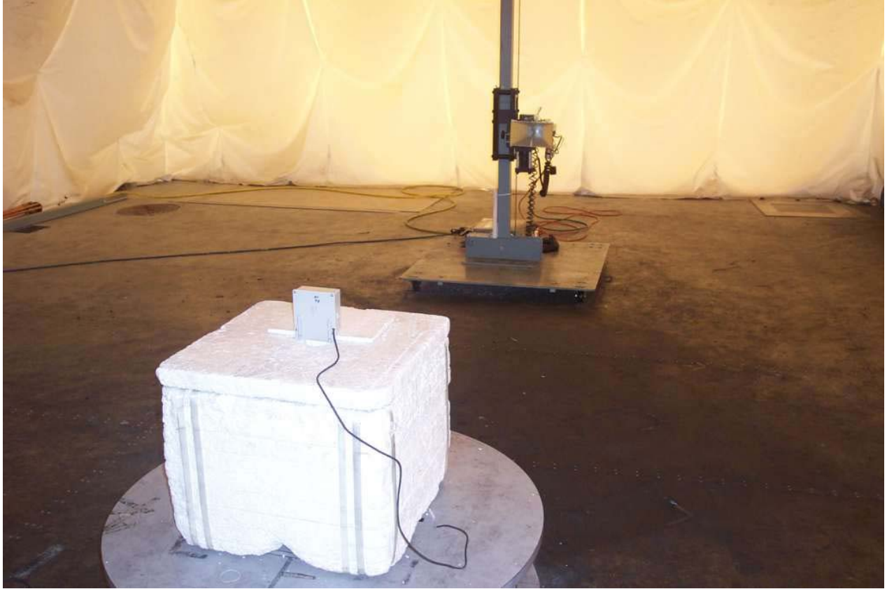
Figure 14: Test setup for radiated spurious emissions below 18GHz with horn antenna in vertical polarity and Remote on turntable
