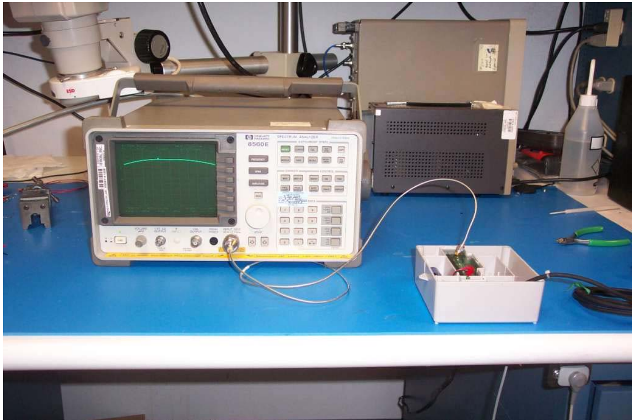
Figure 23: Test Setup for TX conducted power out, 6dB Bandwidth, Bandwidth of Momentary signals (99%BW), TX power spectral density, TX conducted band edge, measurements.
