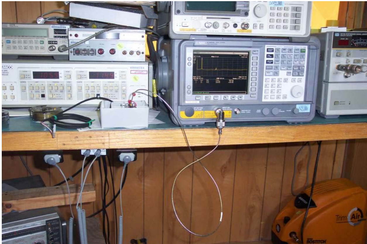
Figure 24. Test setup for TX conducted spurious measurement
