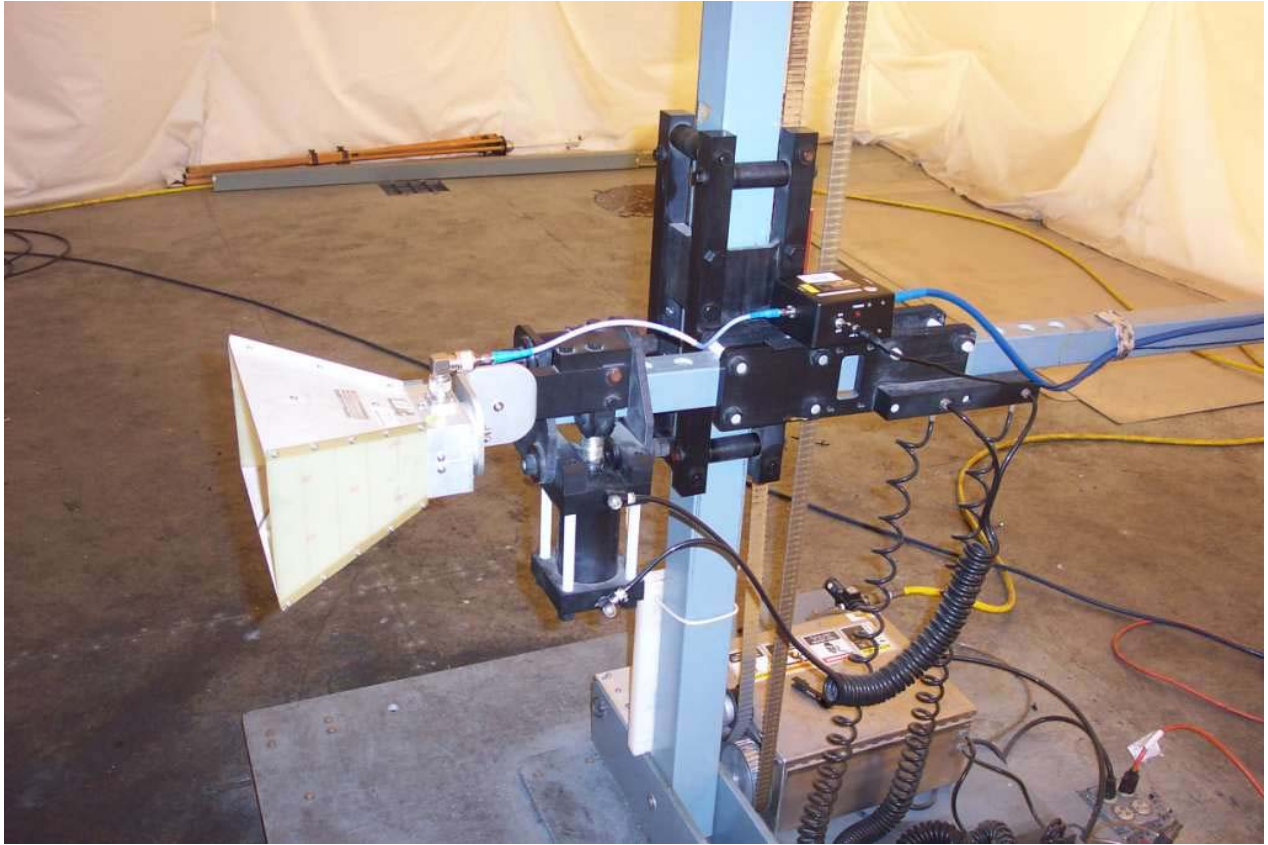
Figure 18: Test setup for RX spurious emission measurements between 1 and 18 GHz with horn in vertical polarity
