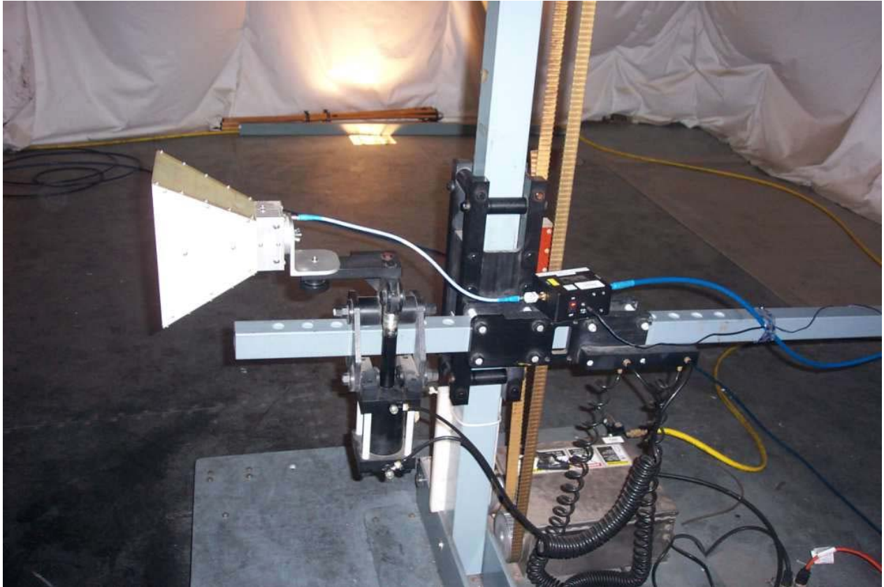
Figure 15: Test setup for TX radiated spurious emissions between 3 and 18GHz (Horizontal polarity shown) with high pass filter
