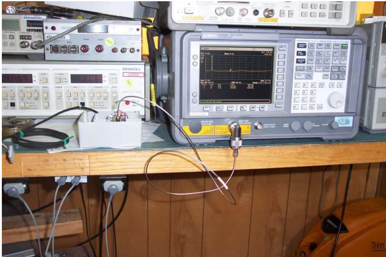
Figure 25: Test setup for TX conducted spurious measurement
