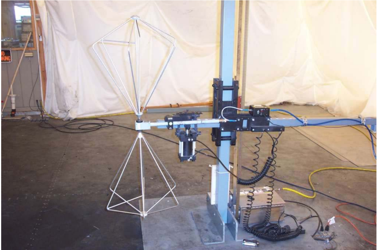
Figure 5: Test Setup for Radiated Spurious measurements between 30MHz and 300MHz using Biconical antenna shown here in vertical orientation
