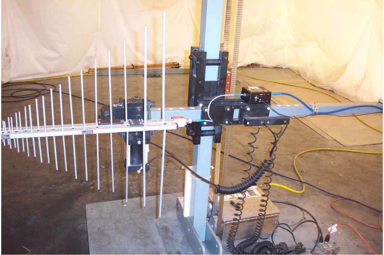
Figure 12: Test setup for RX radiated spurious between 200MHz and 2GHz with Log Periodic in vertical orientation
