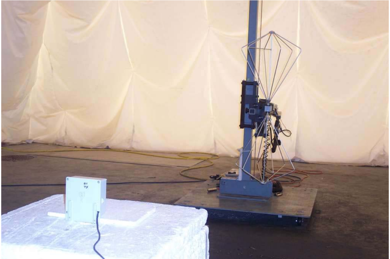
Figure 7: Test Setup for Radiated Spurious measurements between 30MHz and 300MHz using Biconical antenna shown here in vertical orientation and Remote in foreground
