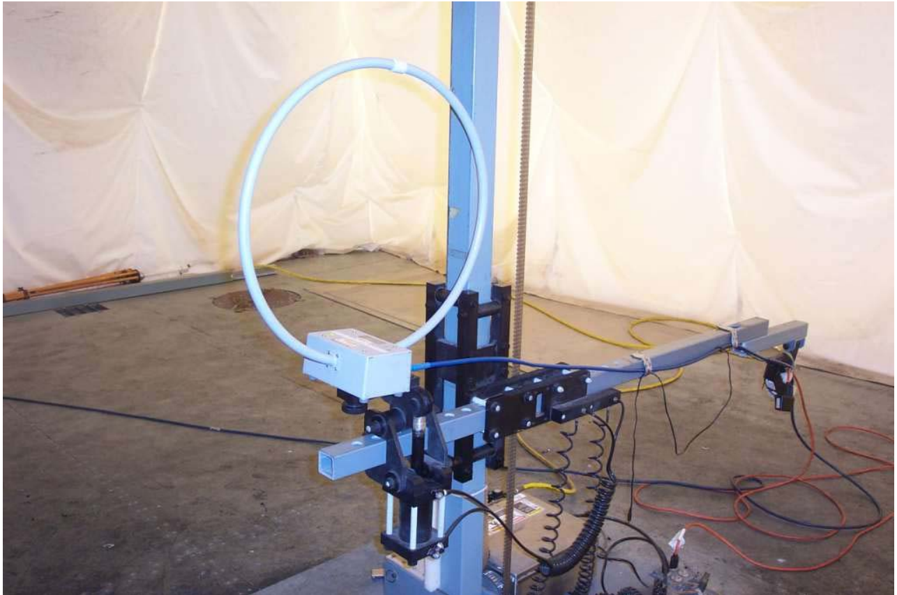
Figure 1: Test setup for radiated spurious between 9kHz and 30MHz with Loop Antenna.
