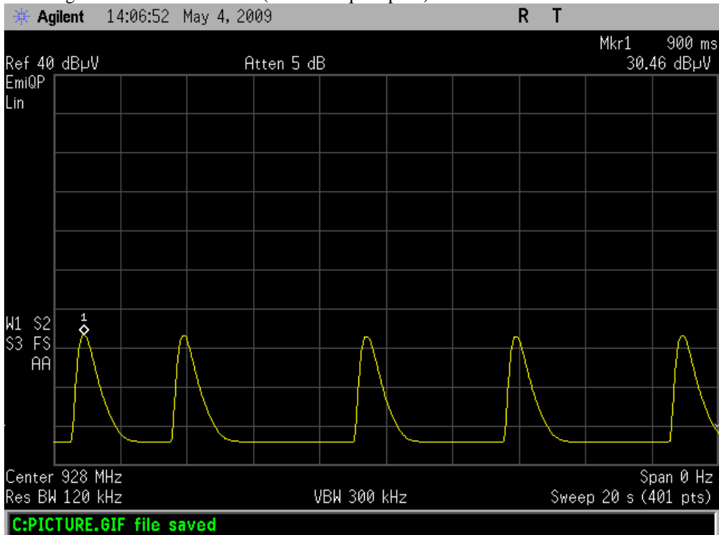
Band edge @ 928MHz conducted (measured quasi peak)
