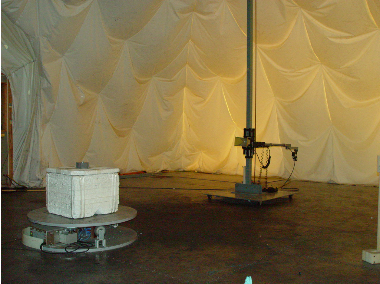
Radiated measurement test setup
