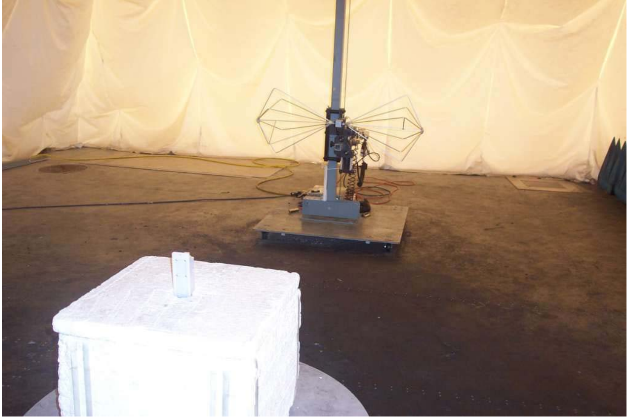
Photo 6: Test Setup for Radiated Spurious measurements between 30MHz and 300MHz using EMCO 3110B Biconical antenna shown here in horizontal orientation and Range Extender in foreground
