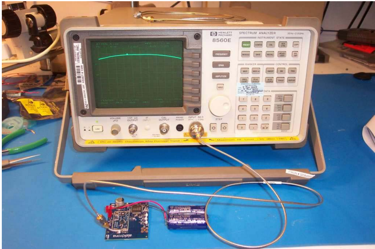
Photo 22: TX conducted measurements (TX conducted power out, 6dB Bandwidth, Bandwidth of Momentary signals (99%BW), TX power spectral density, TX conducted band edge), of Range Extender board using HP8560E Spectrum Analyzer
