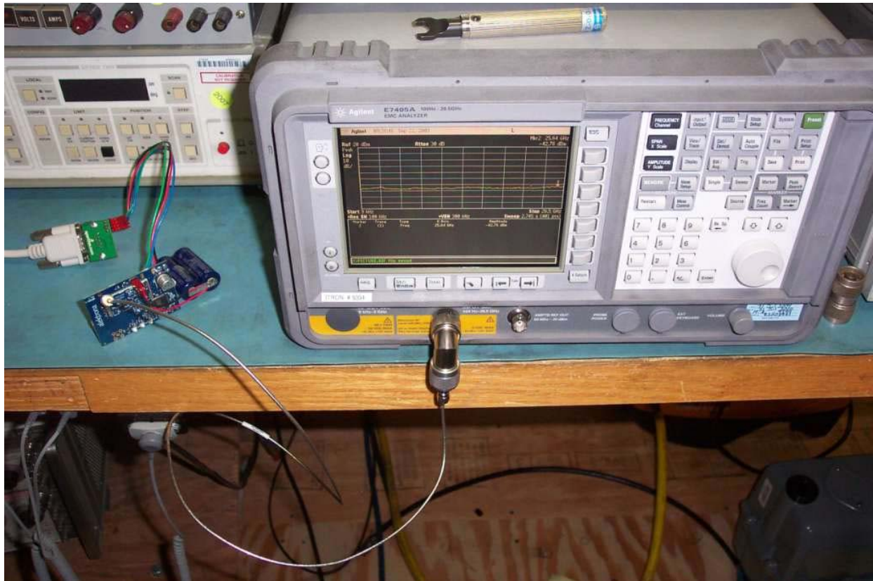
Photo 21: TX conducted spurious measurement with Range Extender board and Agilent E7405A Spectrum Analyzer
