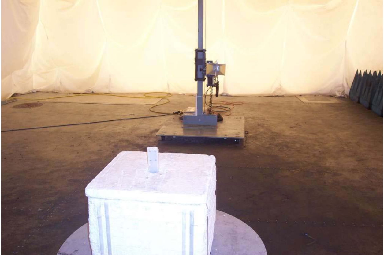
Photo 16: Test setup for radiated spurious emissions between 1 and 18GHz with EMCO 3115 horn antenna in vertical polarity and Range Extender on turntable
