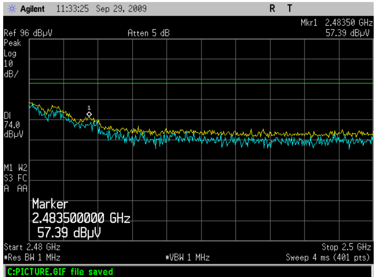
Figure 19: Peak Horizontal Radiated Band Edge (2475MHz Fundamental)
