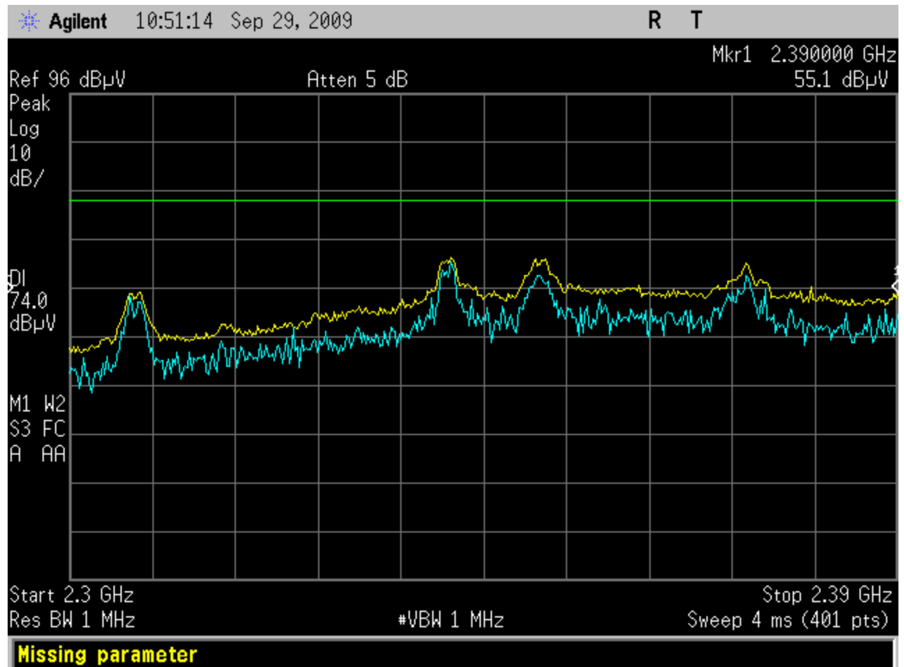
Figure 23: Peak Horizontal Radiated Band Edge (2405MHz Fundamental)
