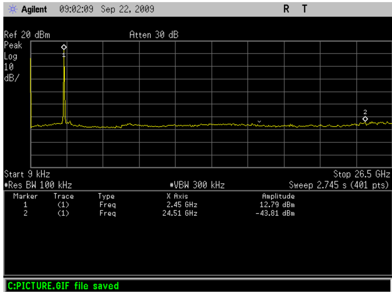
Figure 16: Conducted Spurious Measurement: f=2440MHz
