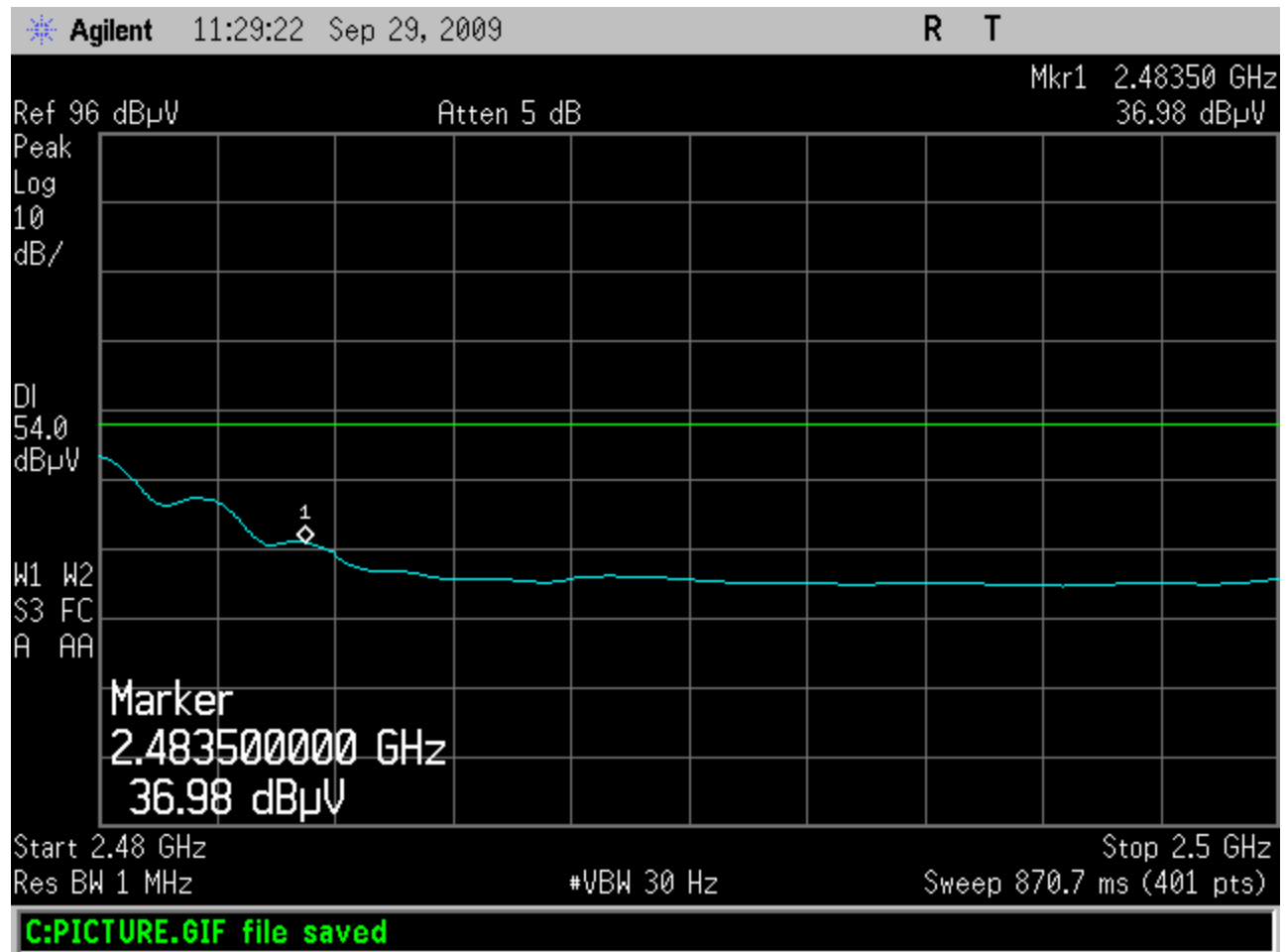
Figure 20: Average Horizontal Radiated Band Edge (2475MHz Fundamental)
