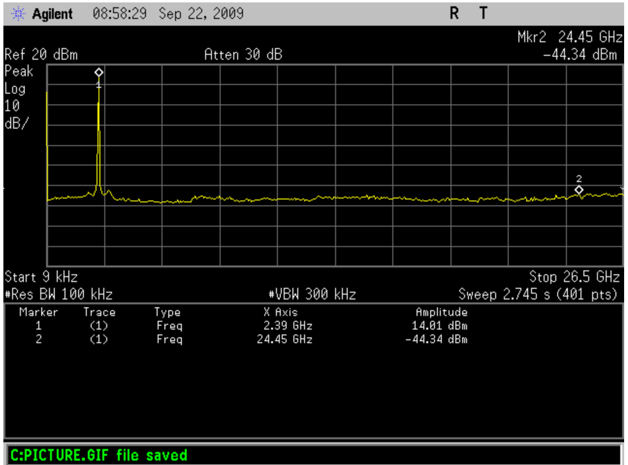
Figure 15: Conducted Spurious Measurement: f=2405MHz
