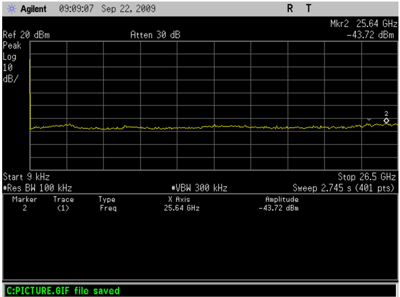
Figure 18: Conducted Spurious Measurement Noise Floor Agilent E7405A
