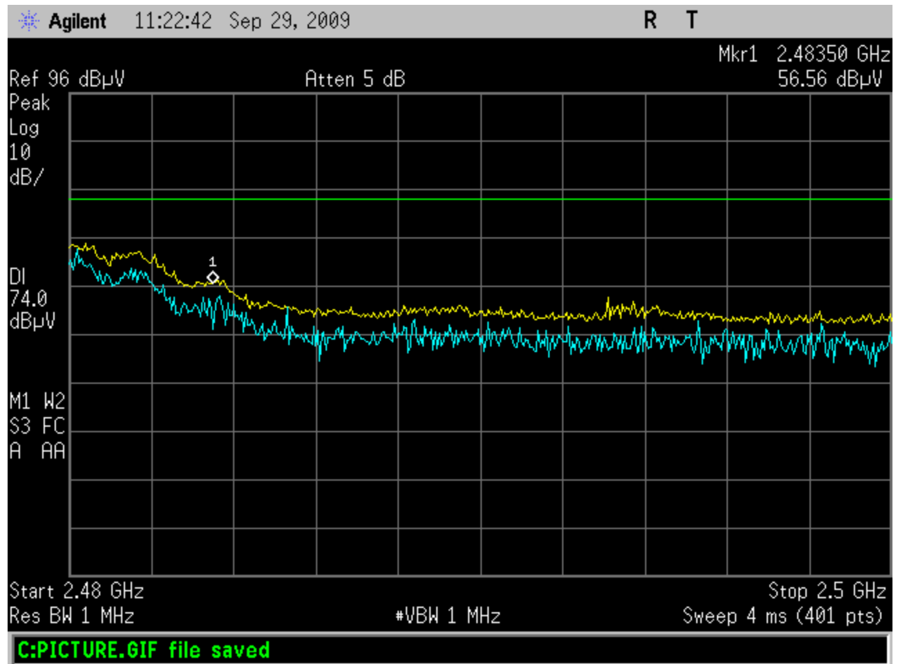
Figure 21: Peak Vertical Radiated Band Edge (2475MHz Fundamental)
