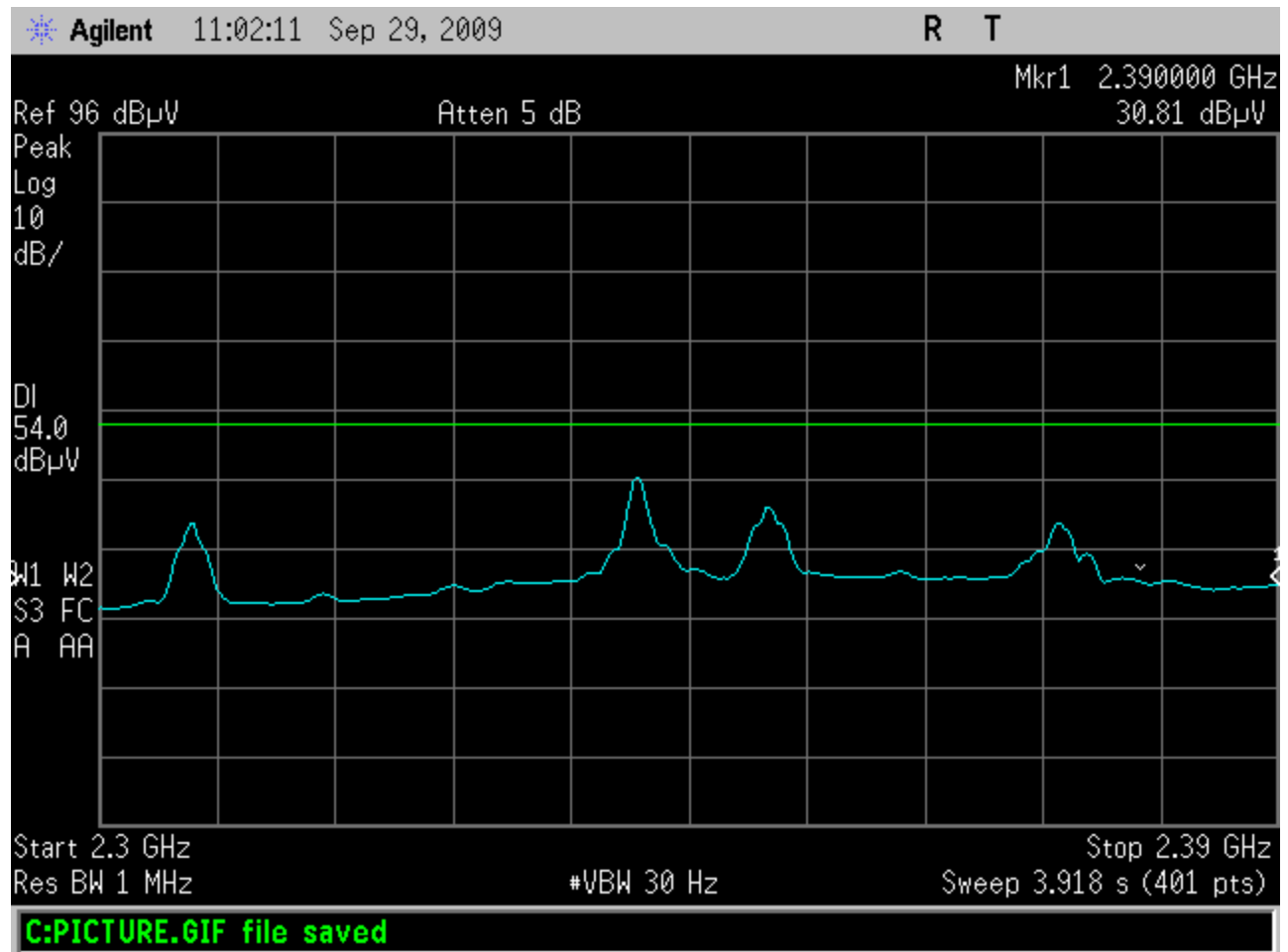
Figure 26: Average Vertical Radiated Band Edge (2405MHz Fundamental)
