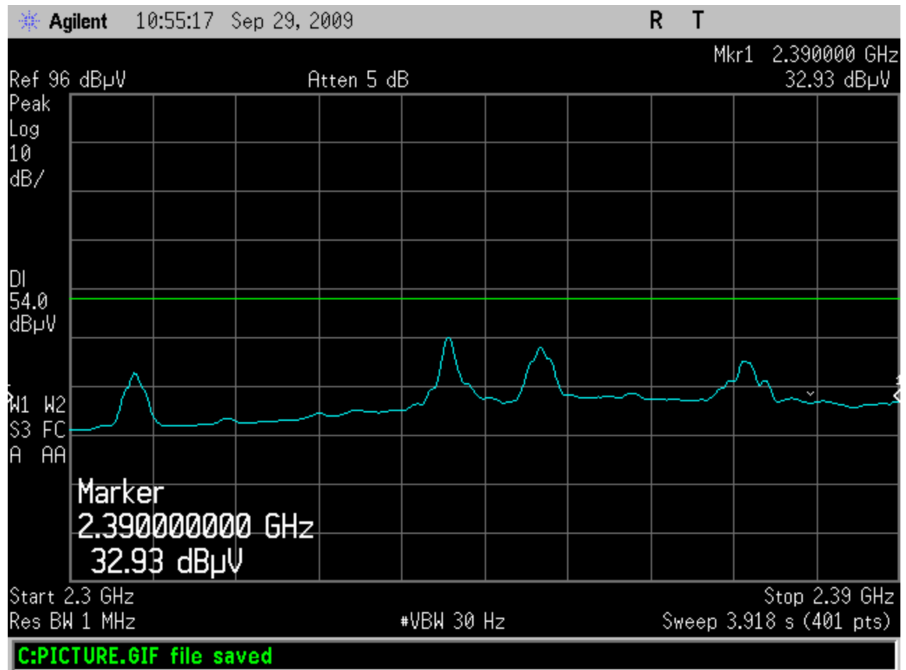
Figure 24: Average Horizontal Radiated Band Edge (2405MHz Fundamental)
