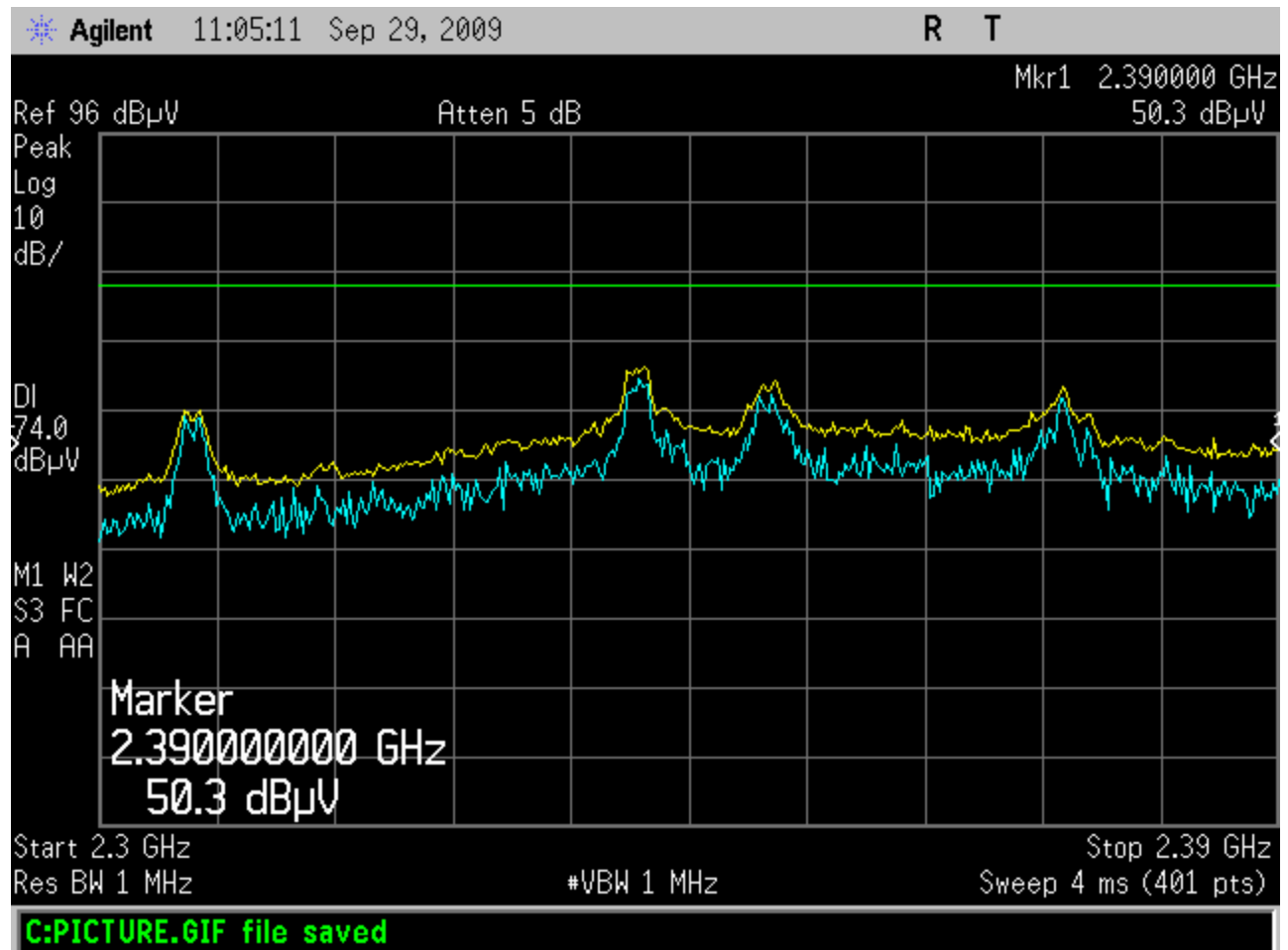
Figure 25: Peak Vertical Radiated Band Edge (2405MHz Fundamental)
