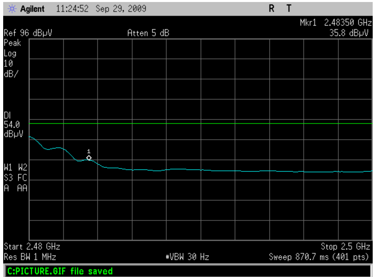
Figure 22: Average Vertical Radiated Band Edge (2475MHz Fundamental)
