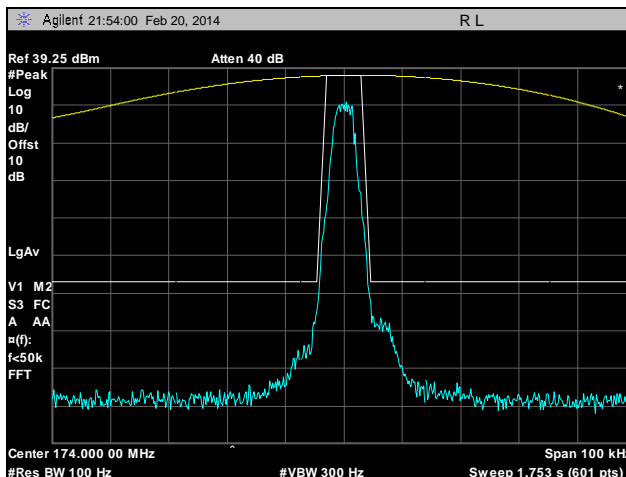
Plot 22. Emission Mask E, High Channel, 174 MHz, 6.25 kHz, High Power
