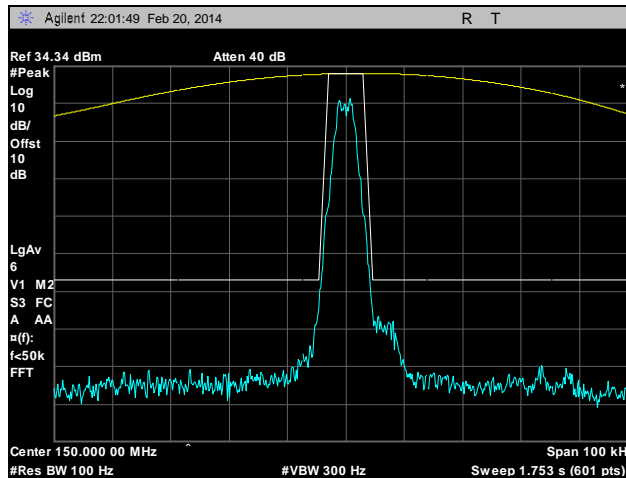
Plot 17. Emission Mask E, Low Channel, 150 MHz, 6.25 kHz, Low Power
