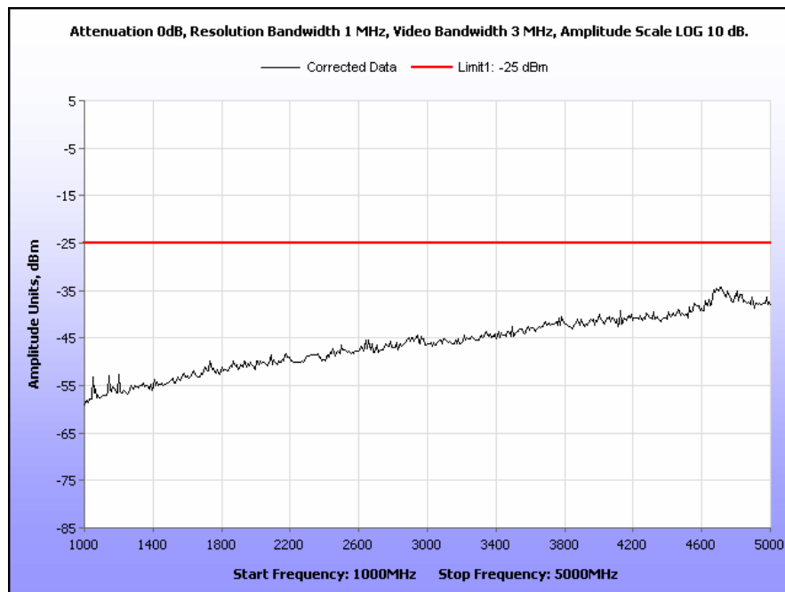
Plot 42. Radiated Spurious Emissions, Low Channel, 6.25 kHz, 1 GHz – 5 GHz
