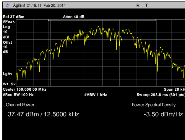
Plot 8. RF Power Output, Low Channel, 150 MHz, 12.5 kHz
