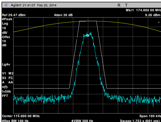
Plot 25. Emission Mask D, High Channel, 174 MHz, 12.5 kHz, Low Power
