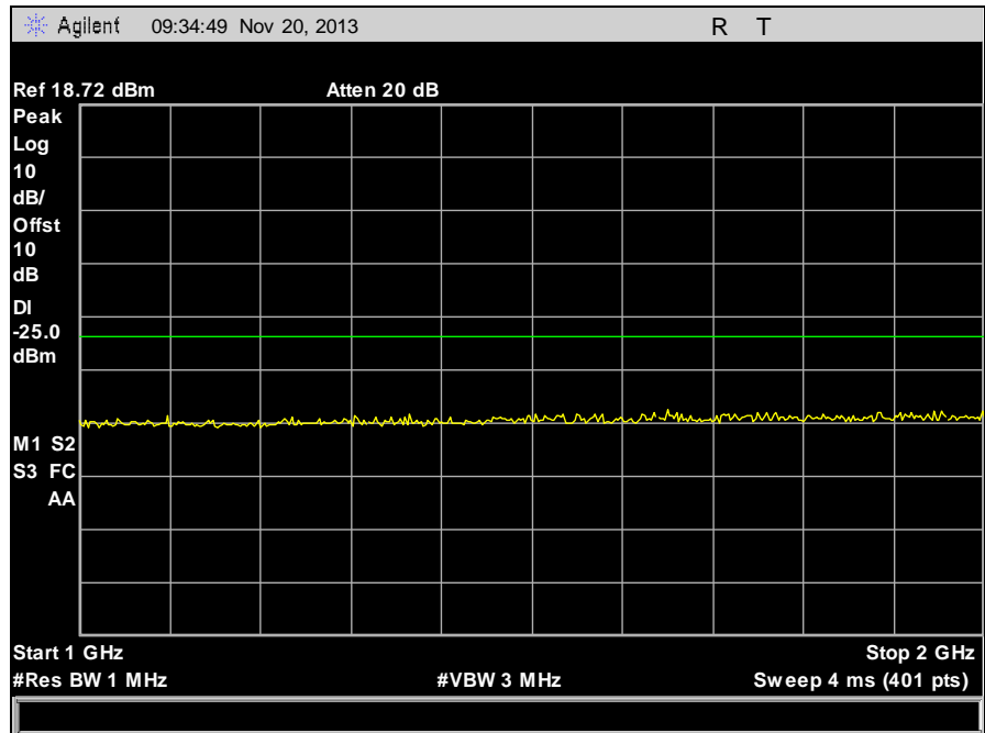
Plot 34. Conducted Spurious Emissions, High Channel, 174 MHz, 6.25 kHz, 1 GHz – 2 GHz
