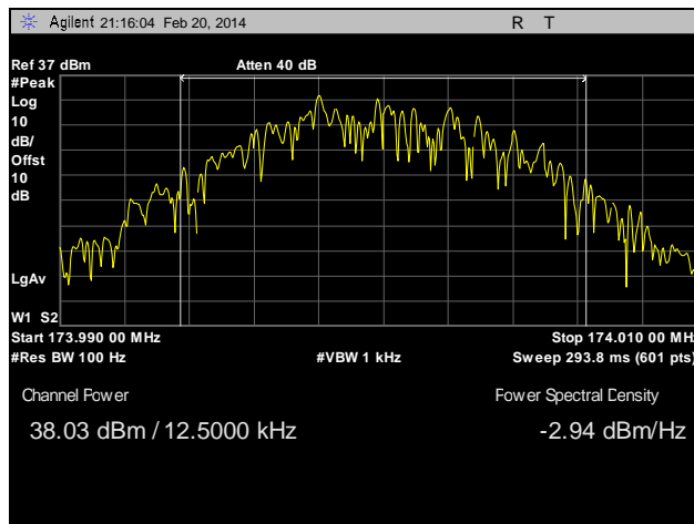
Plot 10. RF Power Output, High Channel, 174 MHz, 12.5 kHz
