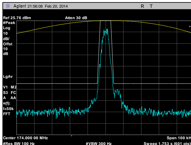
Plot 19. Emission Mask E, High Channel, 174 MHz, 6.25 kHz, Low Power
