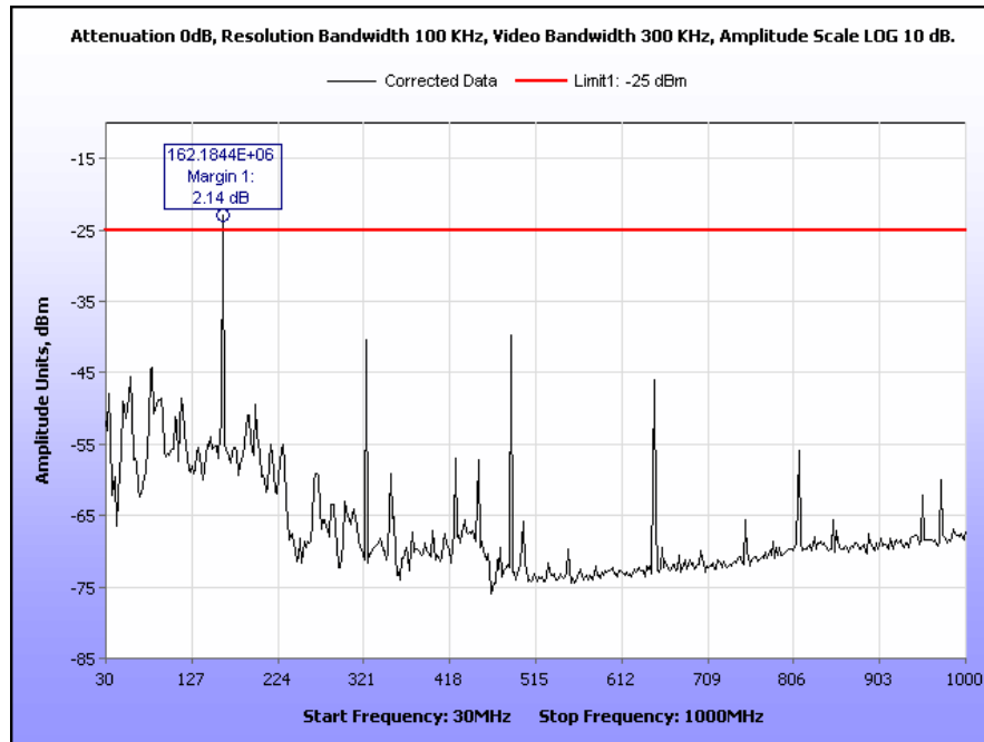
Plot 49. Radiated Spurious Emissions, Mid Channel, 12.5 kHz, 30 MHz – 1 GHz
