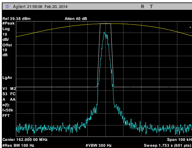
Plot 21. Emission Mask E, Mid Channel, 162 MHz, 6.25 kHz, High Power
