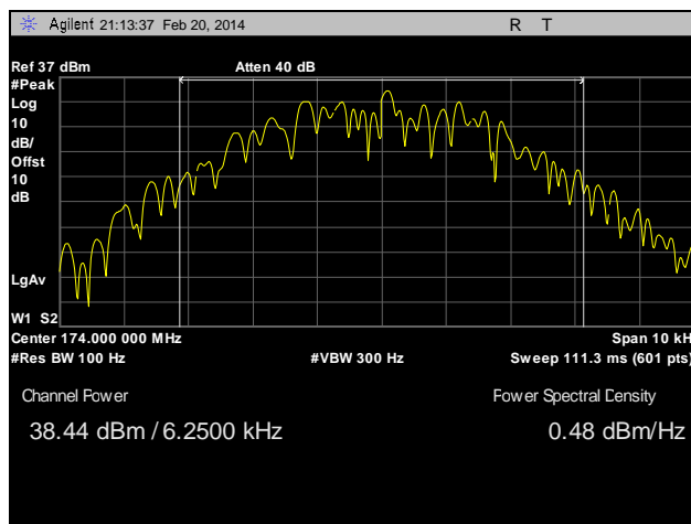
Plot 7. RF Power Output, High Channel, 174 MHz, 6.25 kHz
