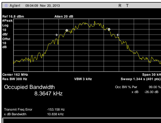
Plot 15. Occupied Bandwidth, Mid Channel, 162 MHz, 12.5 kHz
