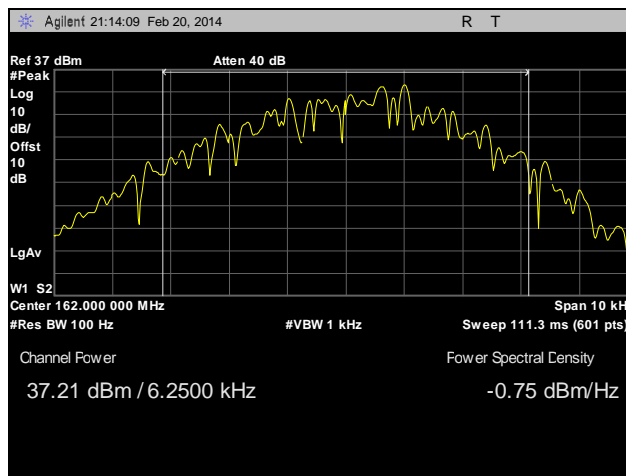
Plot 6. RF Power Output, Mid Channel, 162 MHz, 6.25 kHz
