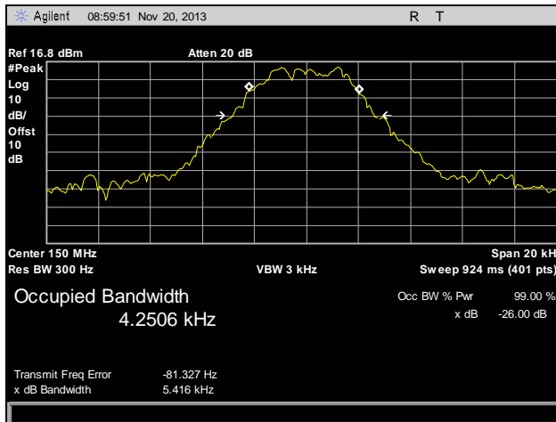
Plot 11. Occupied Bandwidth, Low Channel, 150 MHz, 6.25 kHz
