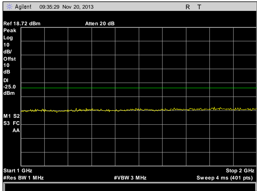
Plot 32. Conducted Spurious Emissions, Mid Channel, 162 MHz, 6.25 kHz, 1 GHz – 2 GHz
