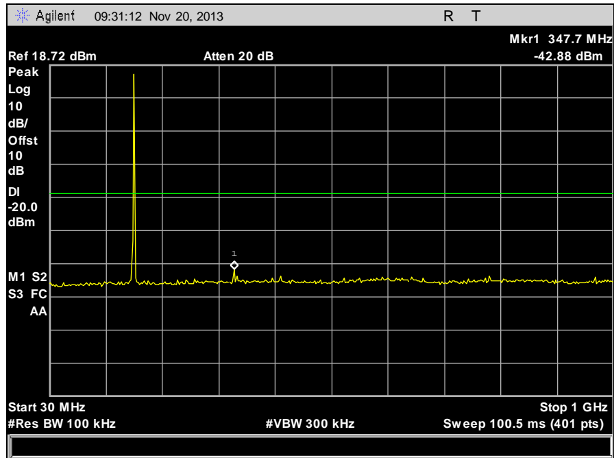
Plot 39. Conducted Spurious Emissions, High Channel, 174 MHz, 12.5 kHz, 30 MHz – 1 GHz
