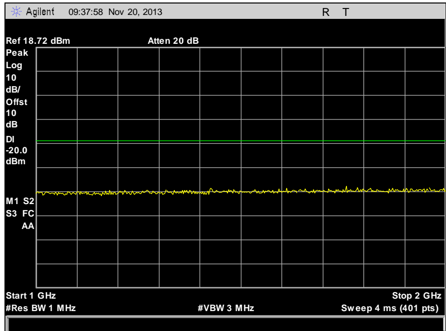
Plot 40. Conducted Spurious Emissions, High Channel, 174 MHz, 12.5 kHz, 1 GHz – 2 GHz
