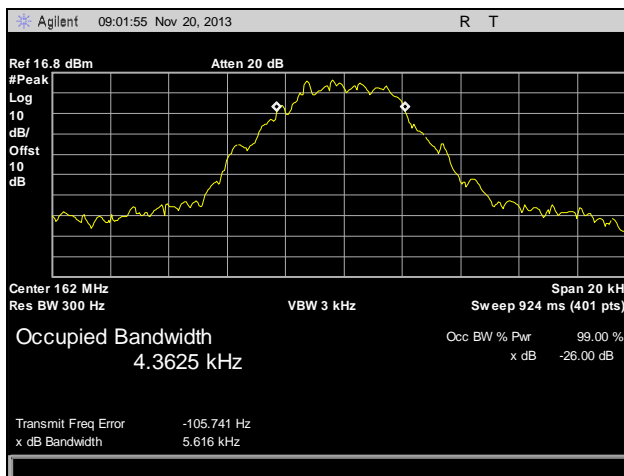
Plot 12. Occupied Bandwidth, Mid Channel, 162 MHz, 6.25 kHz
