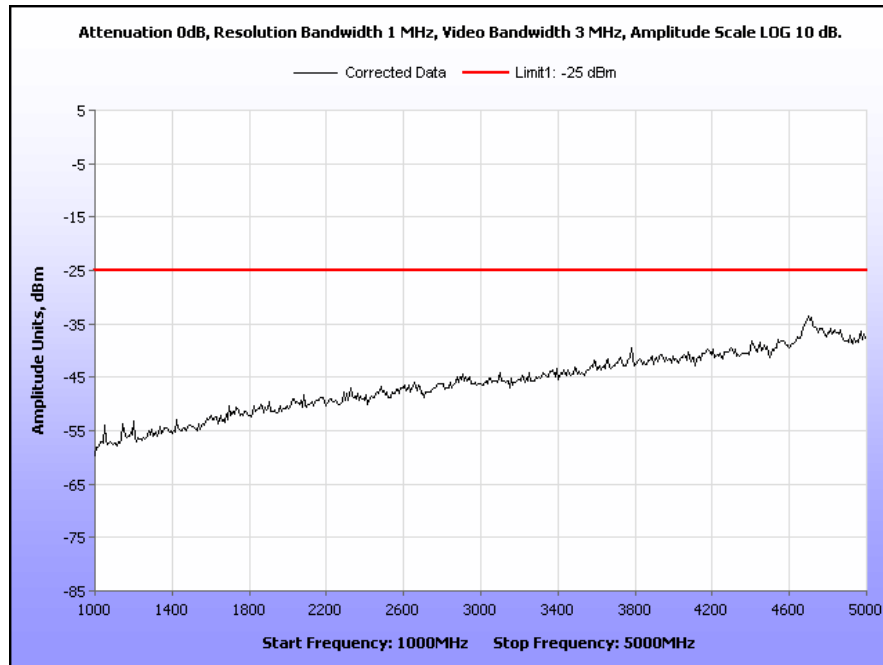
Plot 48. Radiated Spurious Emissions, Low Channel, 12.5 kHz, 1 GHz – 5 GHz
