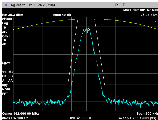
Plot 27. Emission Mask D, Mid Channel, 162 MHz, 12.5 kHz, High Power
