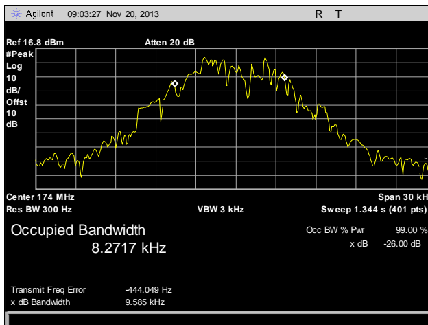
Plot 16. Occupied Bandwidth, High Channel, 174 MHz, 12.5 kHz
