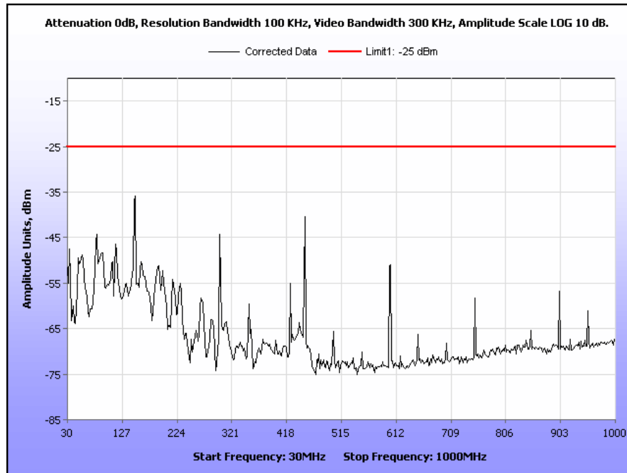
Plot 47. Radiated Spurious Emissions, Low Channel, 12.5 kHz, 30 MHz – 1 GHz
