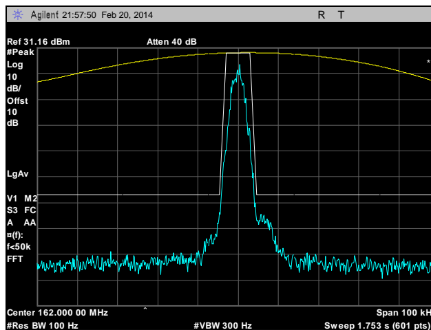
Plot 18. Emission Mask E, Mid Channel, 162 MHz, 6.25 kHz, Low Power
