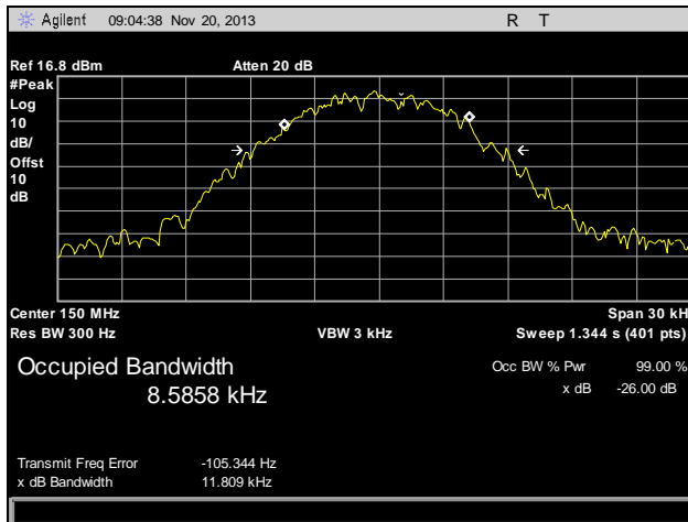
Plot 14. Occupied Bandwidth, Low Channel, 150 MHz, 12.5 kHz
