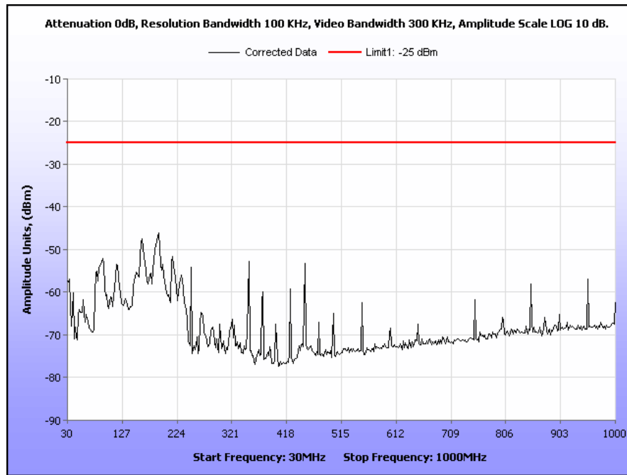
Plot 41. Radiated Spurious Emissions, Low Channel, 6.25 kHz, 30 MHz – 1 GHz
