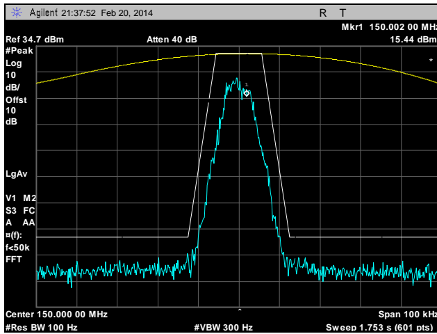
Plot 23. Emission Mask D, Low Channel, 150 MHz, 12.5 kHz, Low Power
