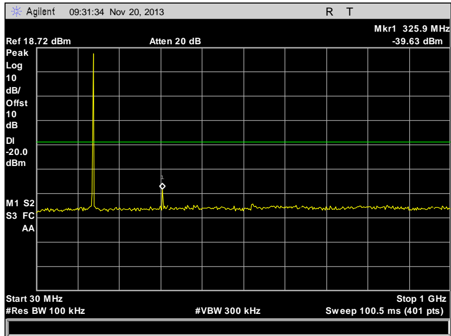
Plot 37. Conducted Spurious Emissions, Mid Channel, 162 MHz, 12.5 kHz, 30 MHz – 1 GHz
