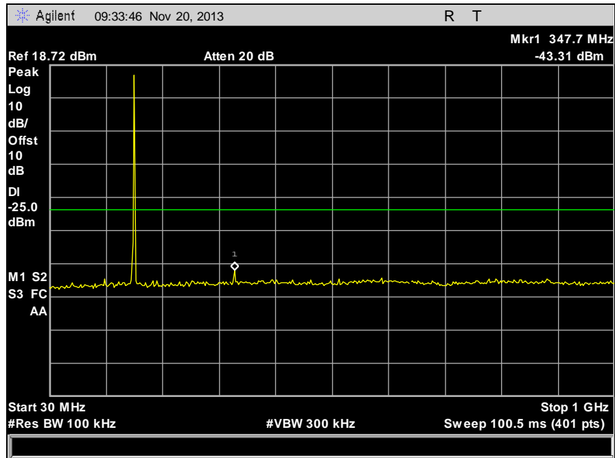
Plot 33. Conducted Spurious Emissions, High Channel, 174 MHz, 6.25 kHz, 30 MHz – 1 GHz
