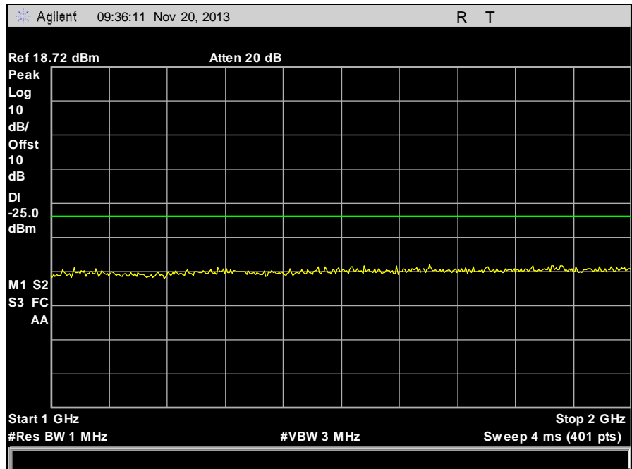
Plot 30. Conducted Spurious Emissions, Low Channel, 150 MHz, 6.25 kHz, 1 GHz – 2 GHz
