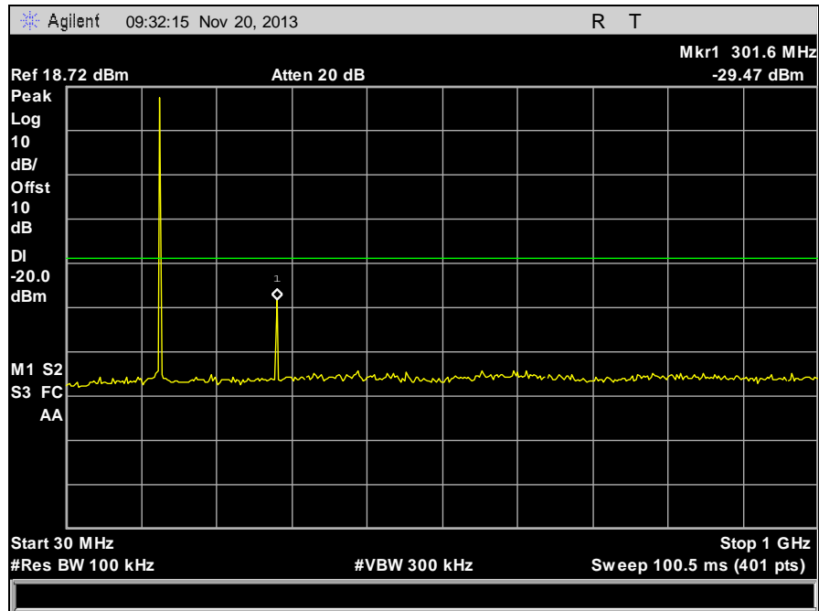
Plot 35. Conducted Spurious Emissions, Low Channel, 150 MHz, 12.5 kHz, 30 MHz – 1 GHz
