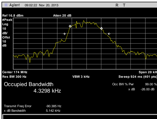
Plot 13. Occupied Bandwidth, High Channel, 174 MHz, 6.25 kHz
