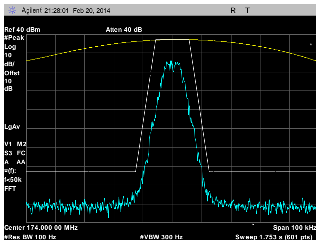
Plot 28. Emission Mask D, High Channel, 174 MHz, 12.5 kHz, High Power
