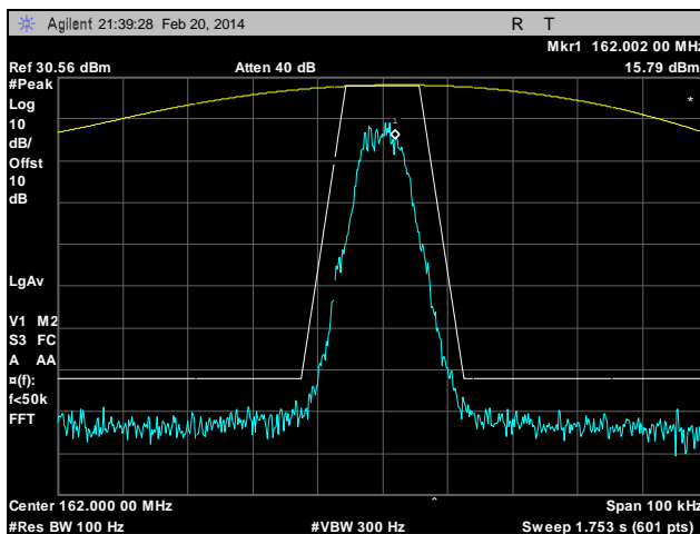
Plot 24. Emission Mask D, Mid Channel, 162 MHz, 12.5 kHz, Low Power
