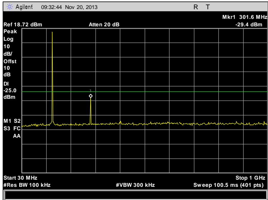
Plot 29. Conducted Spurious Emissions, Low Channel, 150 MHz, 6.25 kHz, 30 MHz – 1 GHz
