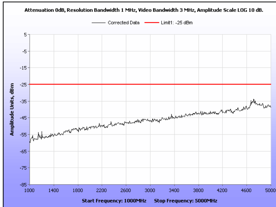
Plot 46. Radiated Spurious Emissions, High Channel, 6.25 kHz, 1 GHz – 5 GHz
