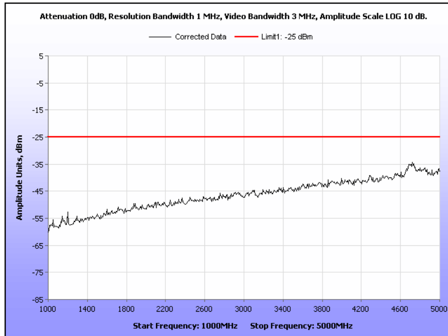
Plot 44. Radiated Spurious Emissions, Mid Channel, 6.25 kHz, 1 GHz – 5 GHz
