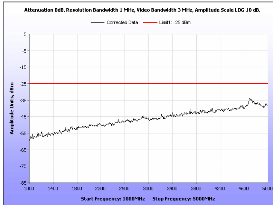
Plot 52. Radiated Spurious Emissions, High Channel, 12.5 kHz, 1 GHz – 5 GHz
