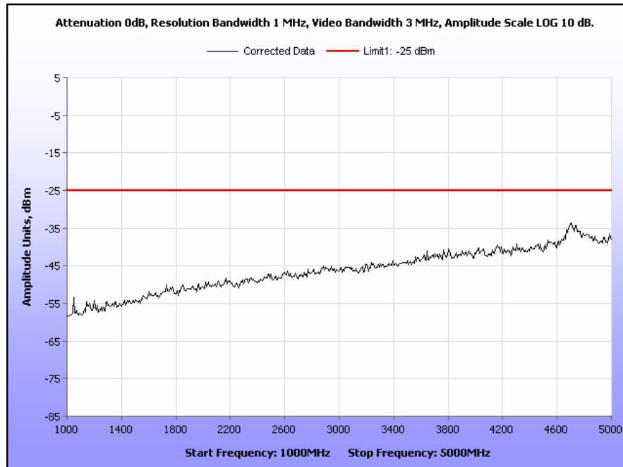
Plot 50. Radiated Spurious Emissions, Mid Channel, 12.5 kHz, 1 GHz – 5 GHz
