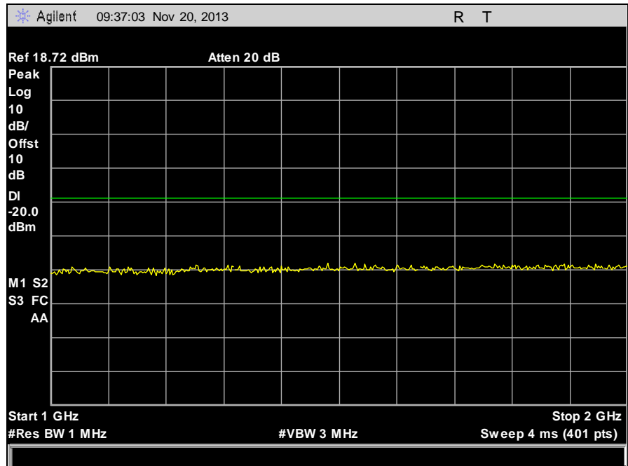
Plot 36. Conducted Spurious Emissions, Low Channel, 150 MHz, 12.5 kHz, 1 GHz – 2 GHz
