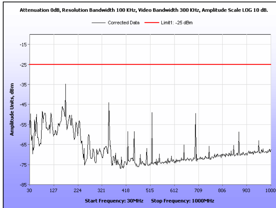
Plot 45. Radiated Spurious Emissions, High Channel, 6.25 kHz, 30 MHz – 1 GHz
