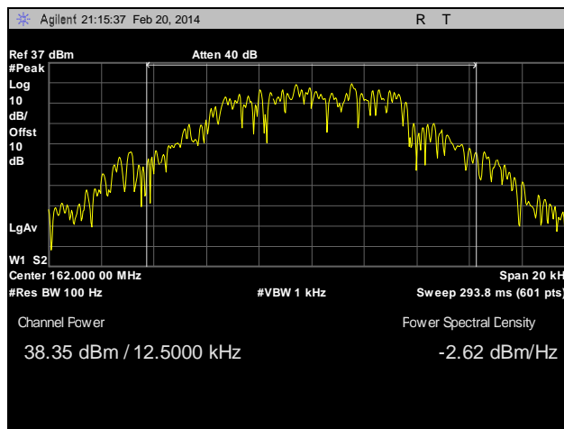
Plot 9. RF Power Output, Mid Channel, 162 MHz, 12.5 kHz
