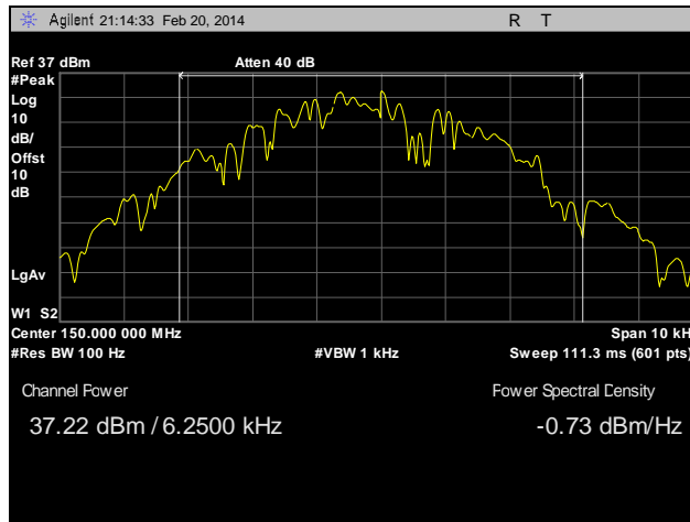
Plot 5. RF Power Output, Low Channel, 150 MHz, 6.25 kHz
