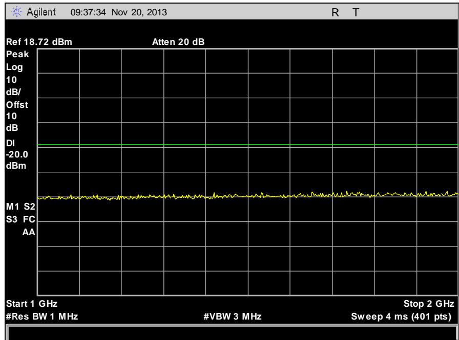
Plot 38. Conducted Spurious Emissions, Mid Channel, 162 MHz, 12.5 kHz, 1 GHz – 2 GHz
