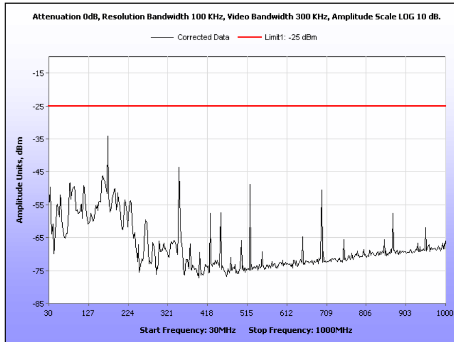
Plot 51. Radiated Spurious Emissions, High Channel, 12.5 kHz, 30 MHz – 1 GHz
