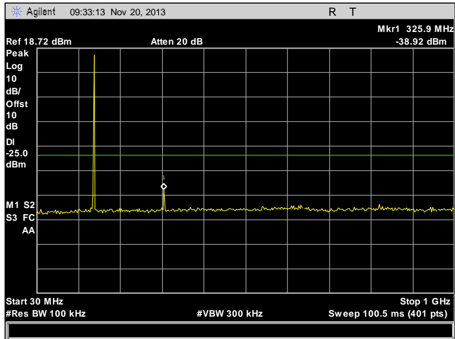
Plot 31. Conducted Spurious Emissions, Mid Channel, 162 MHz, 6.25 kHz, 30 MHz – 1 GHz
