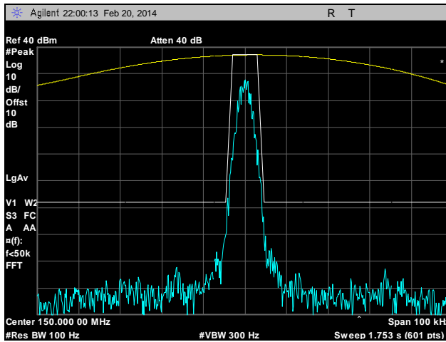
Plot 20. Emission Mask E, Low Channel, 150 MHz, 6.25 kHz, High Power
