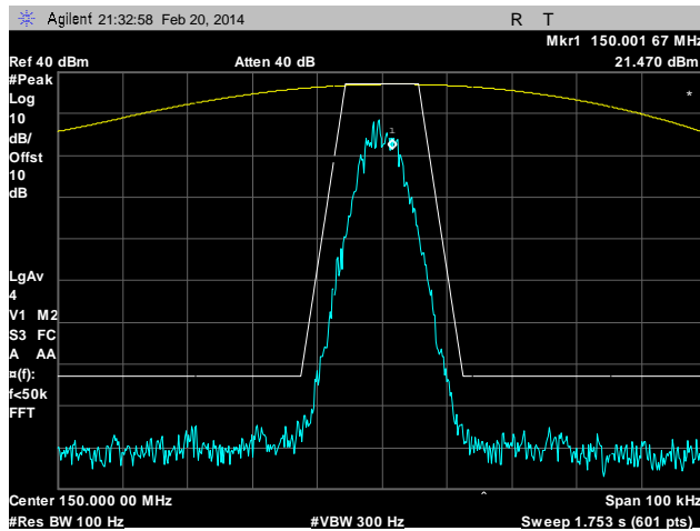
Plot 26. Emission Mask D, Low Channel, 150 MHz, 12.5 kHz, High Power
