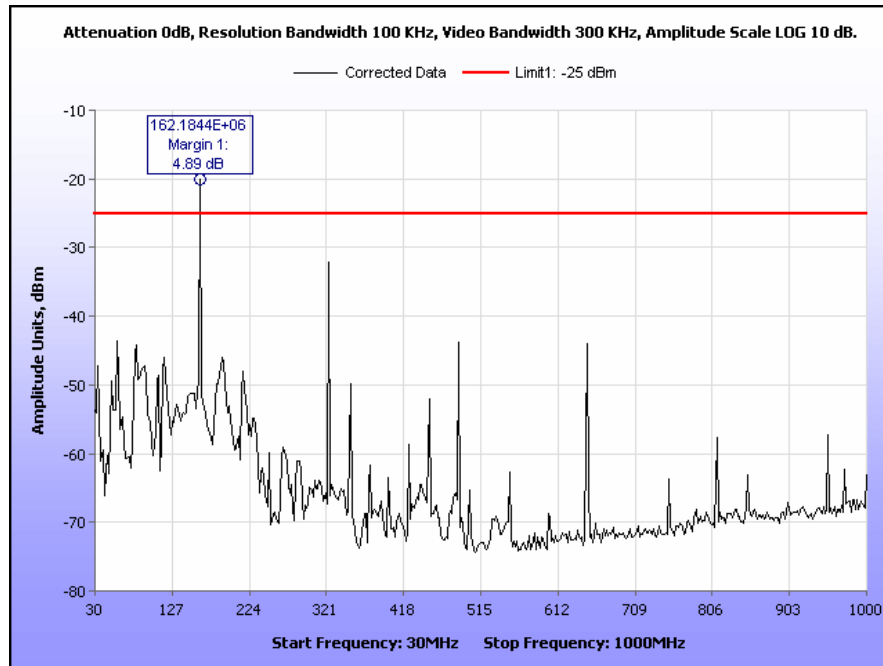
Plot 43. Radiated Spurious Emissions, Mid Channel, 6.25 kHz, 30 MHz – 1 GHz
