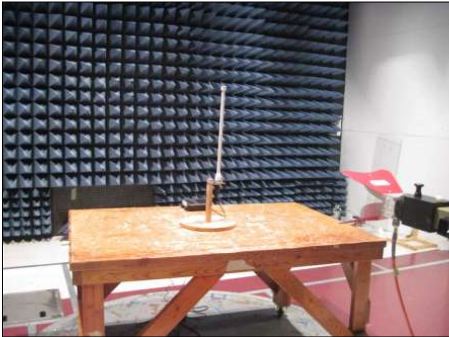
Photograph 12. Radiated Spurious Emissions, Test Setup, Omni Antenna, Above 1 GHz
