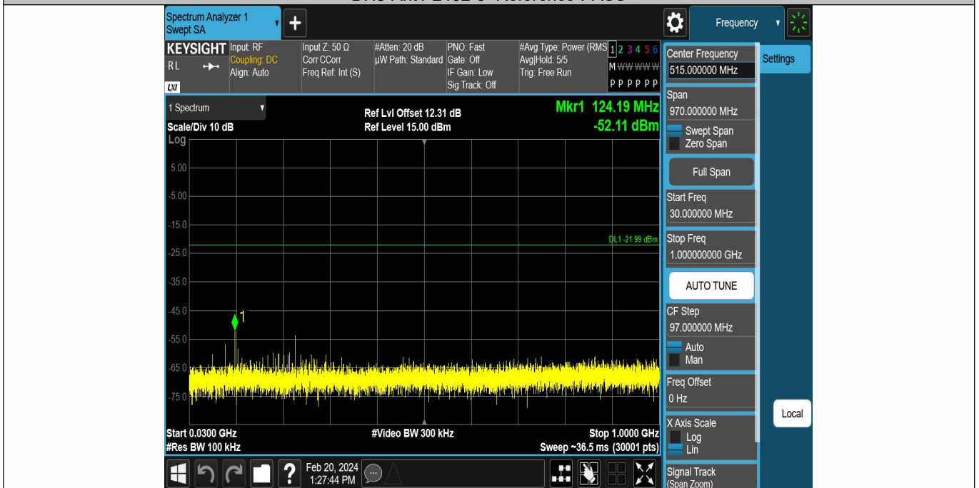
DH5-Ant1-2402-30~1000-PASS
