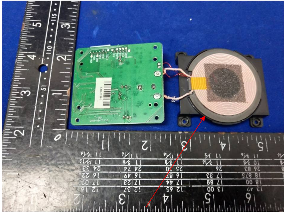
WPT Coil
