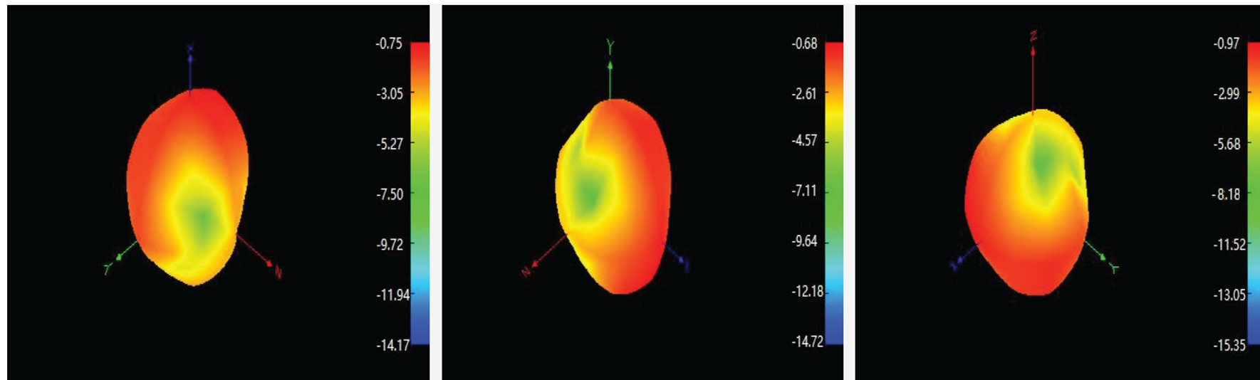
3D Radiation Pattern for 2440MHz
