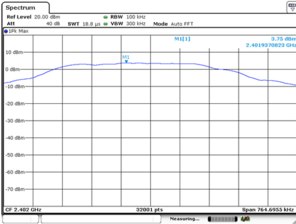
PSD 100kHz Plot: Channel 00
