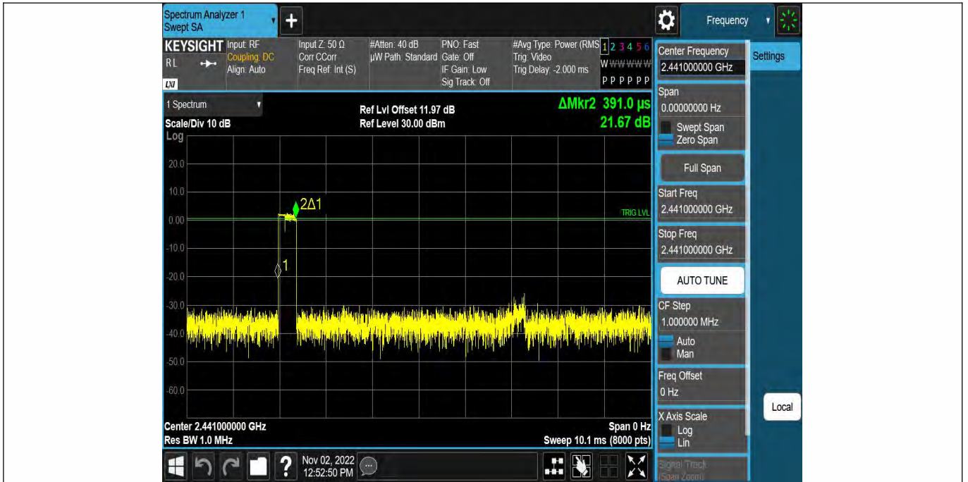
3DH1-Ant1-Hop-0.391-320
