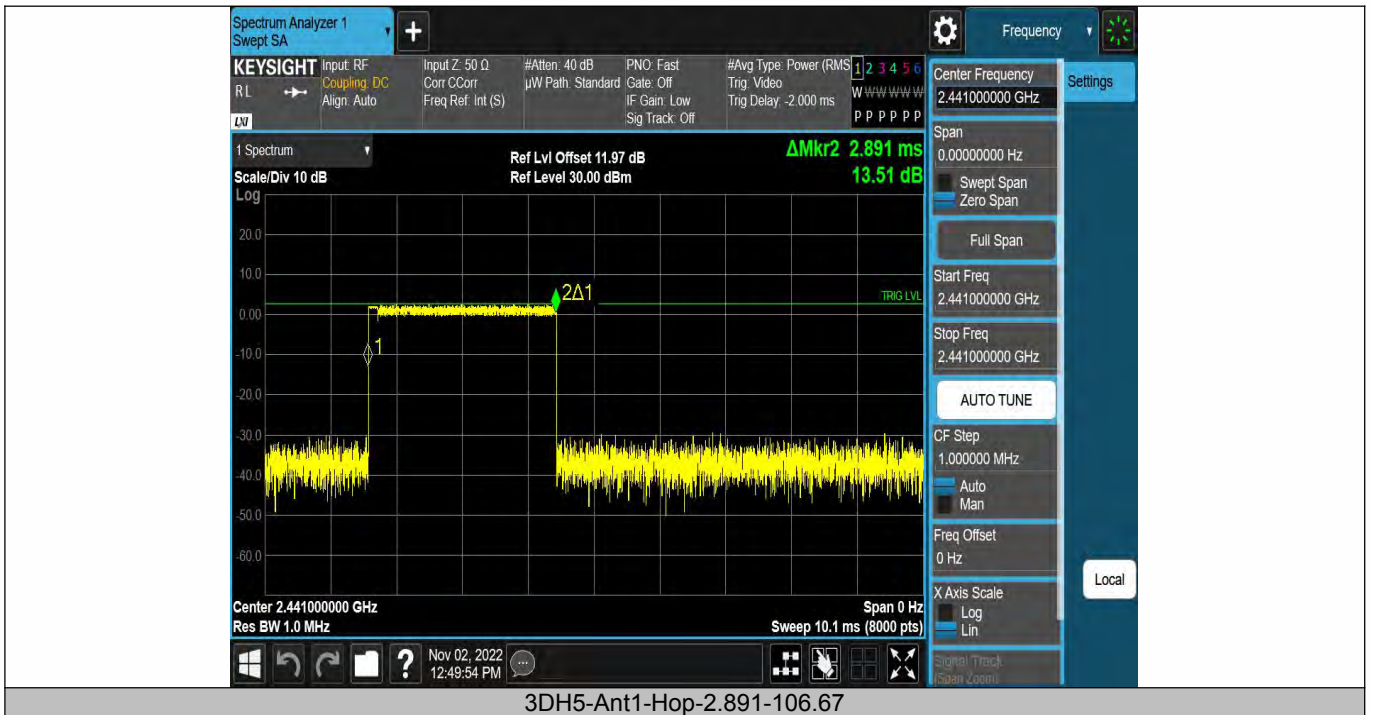
3DH5-Ant1-Hop-2.891-106.67
