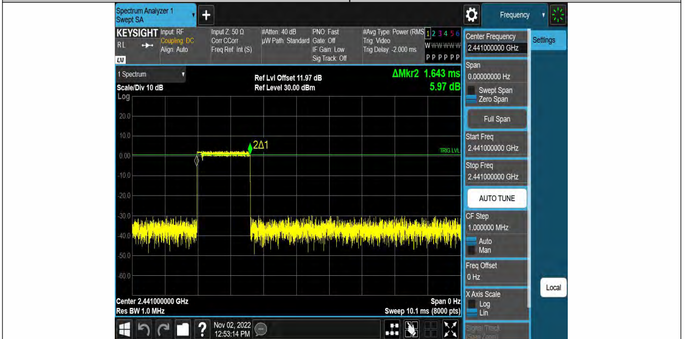
3DH3-Ant1-Hop-1.643-160
