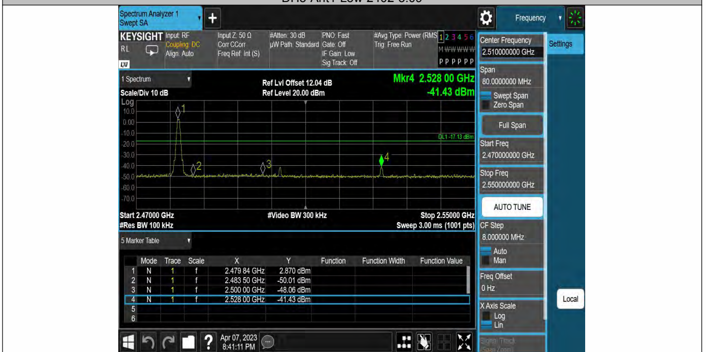
DH5-Ant1-High-2480-2.87
