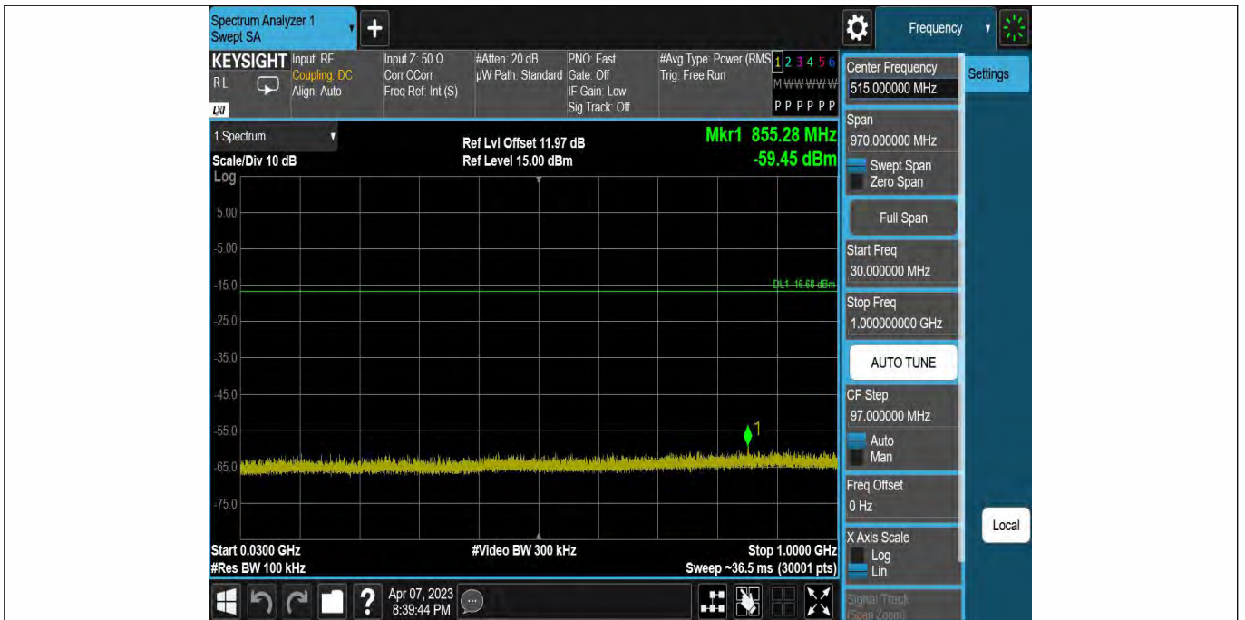
DH5-Ant1-2441-30~1000-3.32
