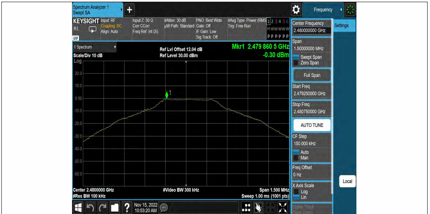
DH5-Ant1-2480-0~Reference--0.30
