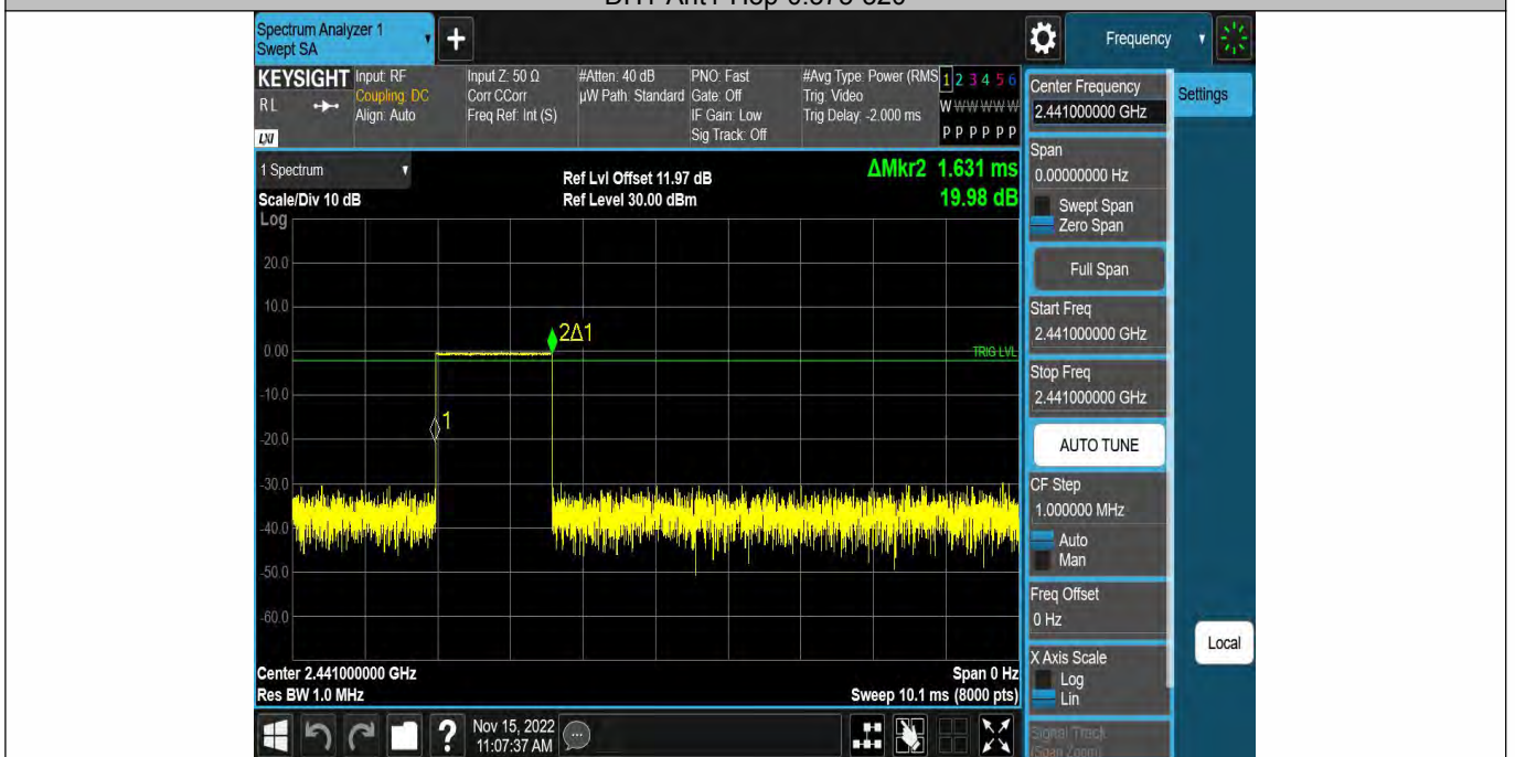
DH3-Ant1-Hop-1.631-160
