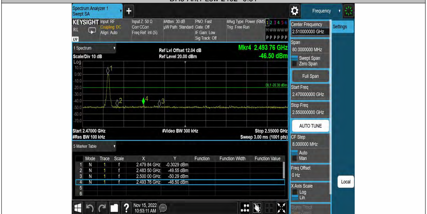
DH5-Ant1-High-2480--0.30
