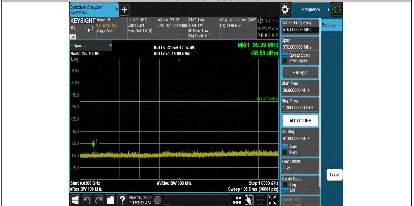
DH5-Ant1-2480-30~1000--0.30
