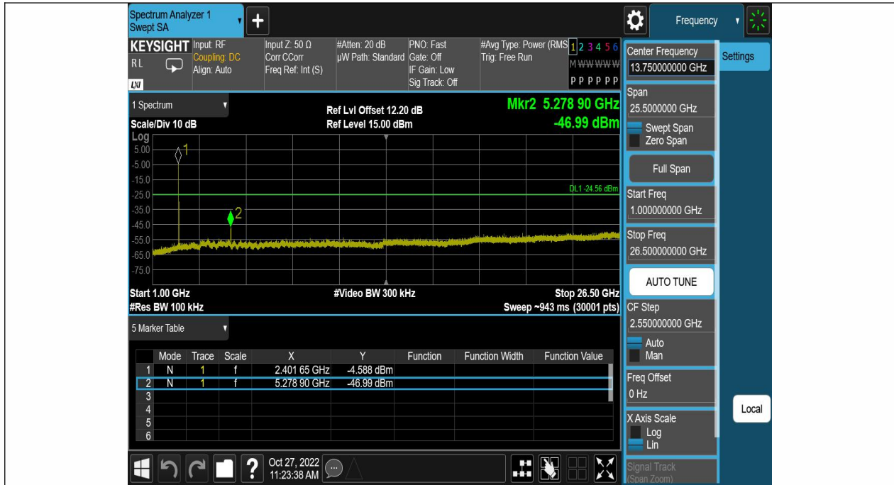
BLE_1M-Ant1-2402-1000~26500--4.56
