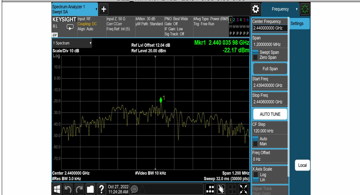
BLE_1M-Ant1-2440--22.17-0.00-0.00-0.00
