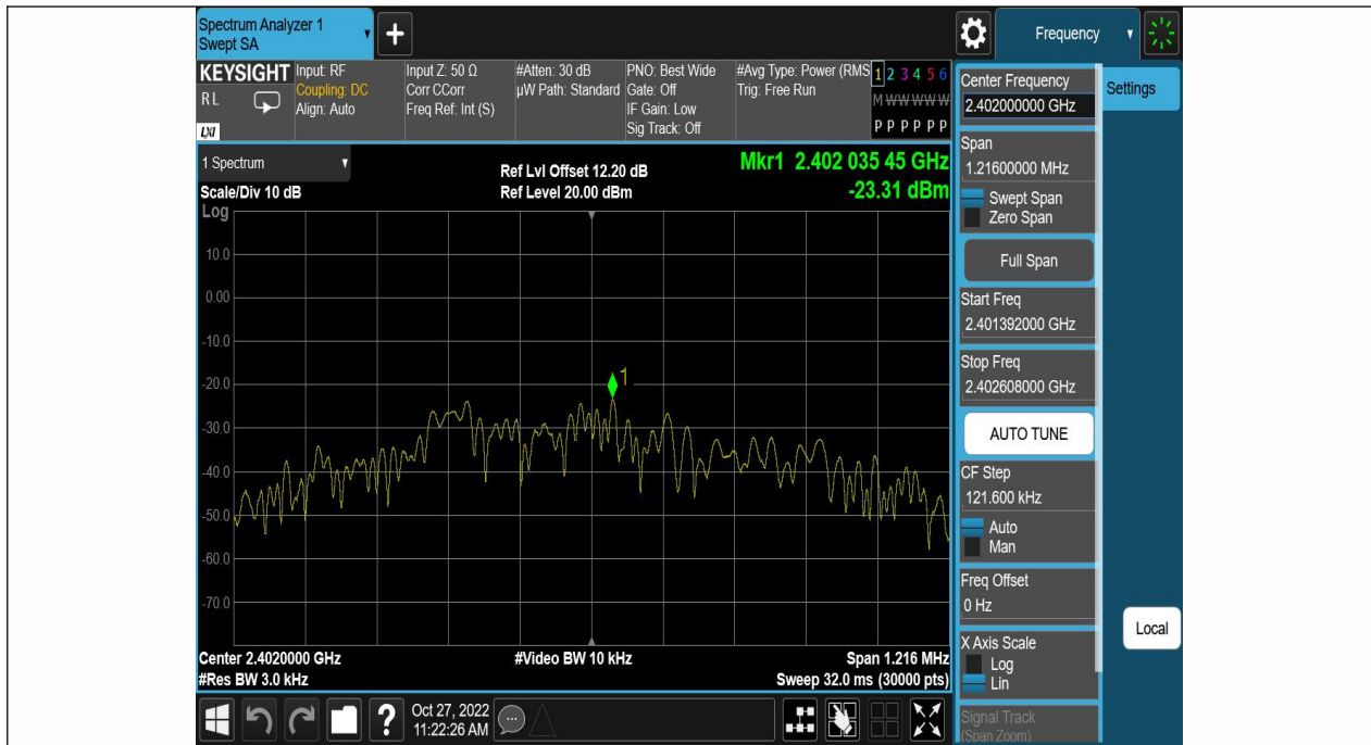
BLE_1M-Ant1-2402--23.31-0.00-0.00-0.00
