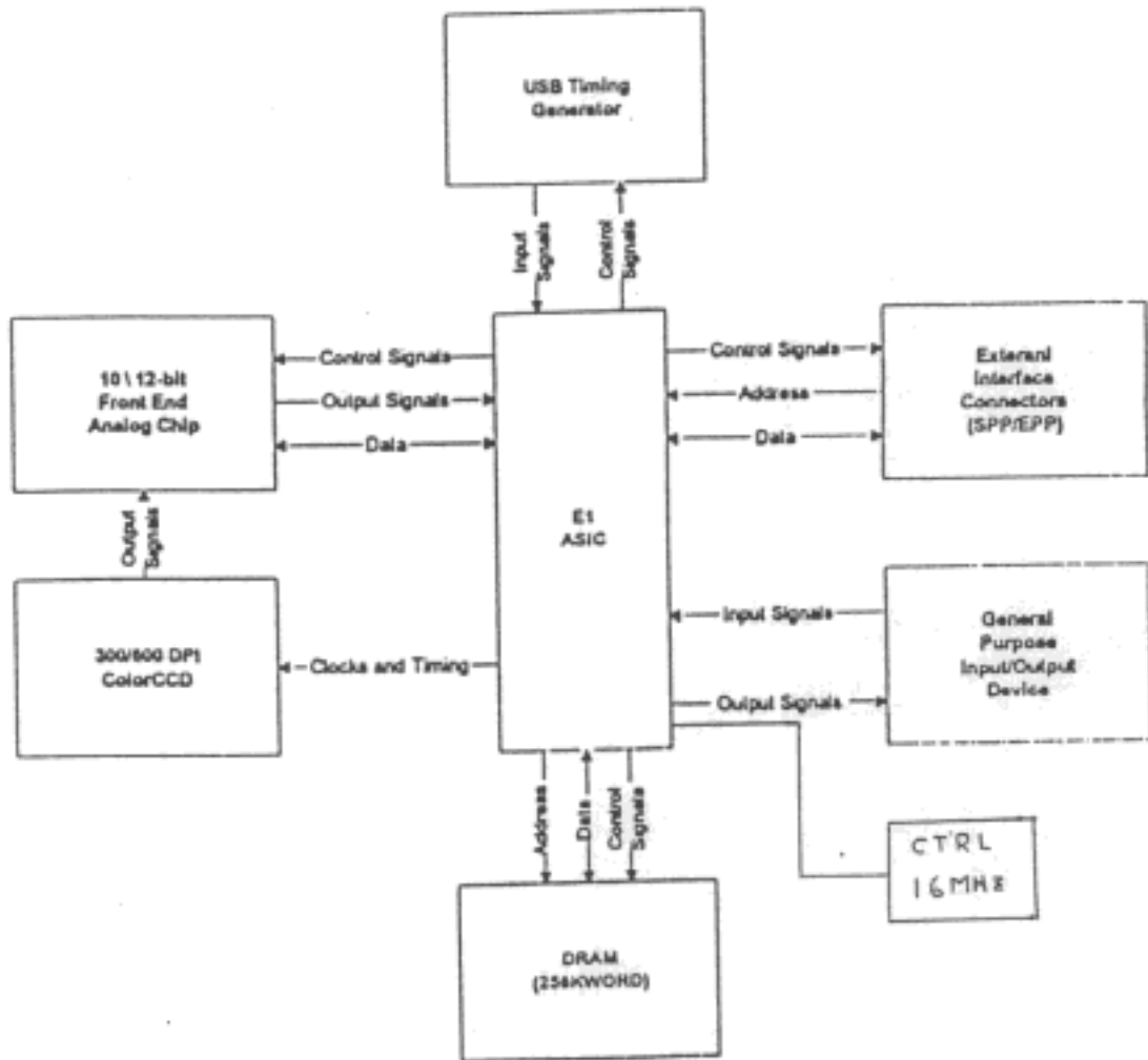
• The Block Diagram of Flat Bed Scanner
