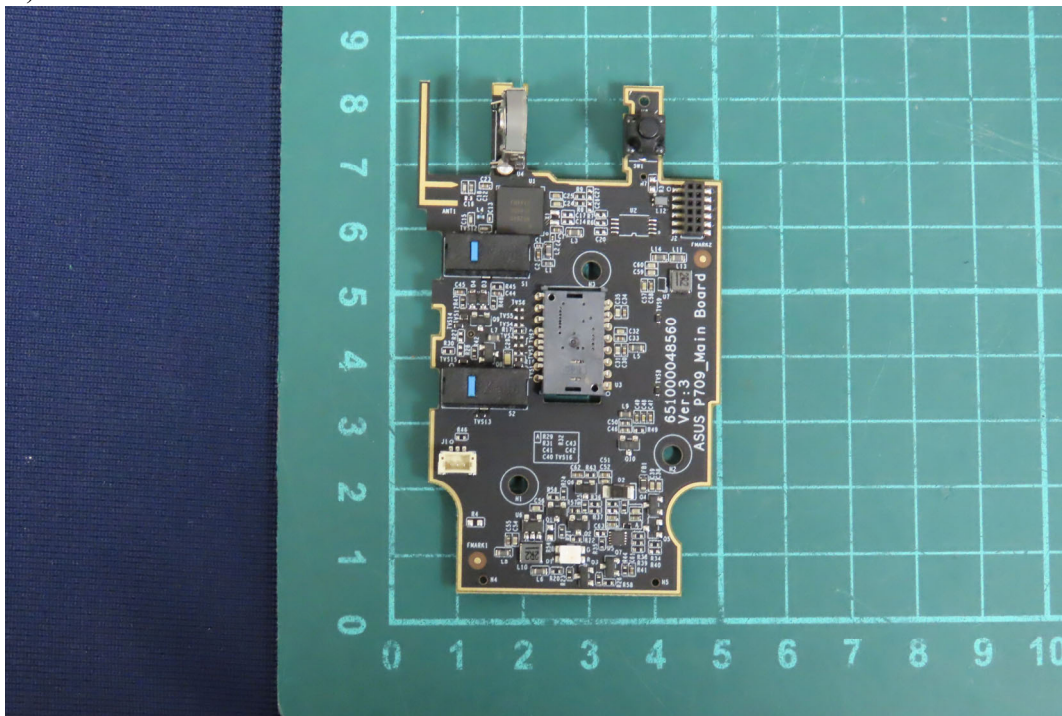
(11) EUT Photo
