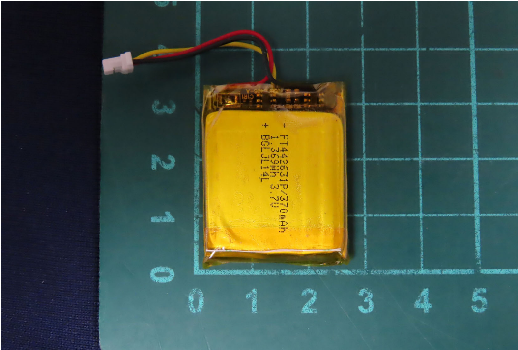
(5) EUT Photo - Battery - MFR: Hangzhou Future Power Technology Co., Ltd. Model No.: FT442631P/370mAh
