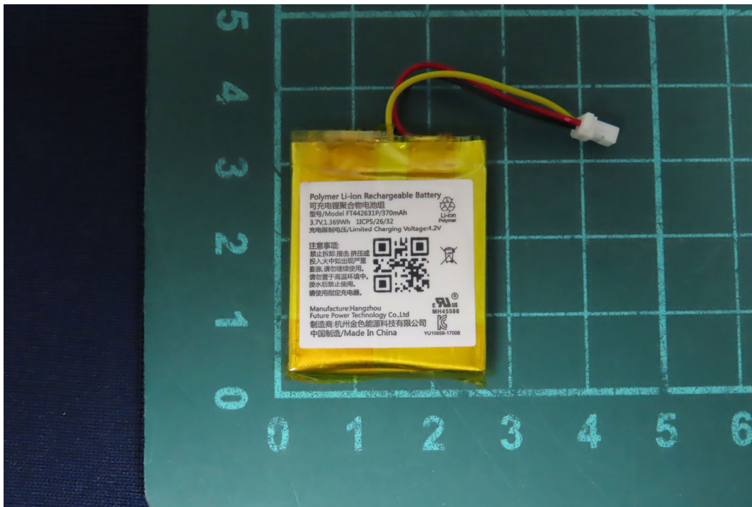
(4) EUT Photo - Battery - MFR: Hangzhou Future Power Technology Co., Ltd.
