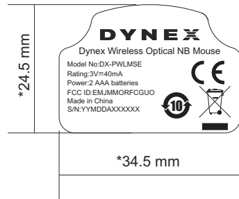
DX-PWLMSE Mouse label SCALE: 1:1
