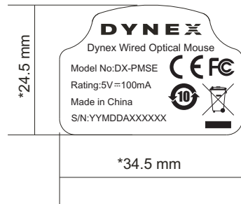
DX-PMSE Mouse label SCALE: 1:1
