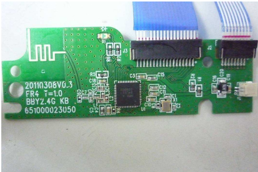
Fig. 4: Internal view
