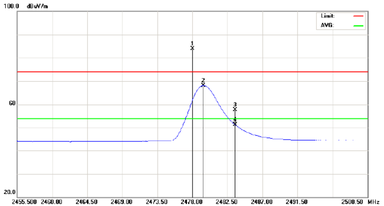
TX CH 77 (Restricted Bands Requirements, Vertical)
