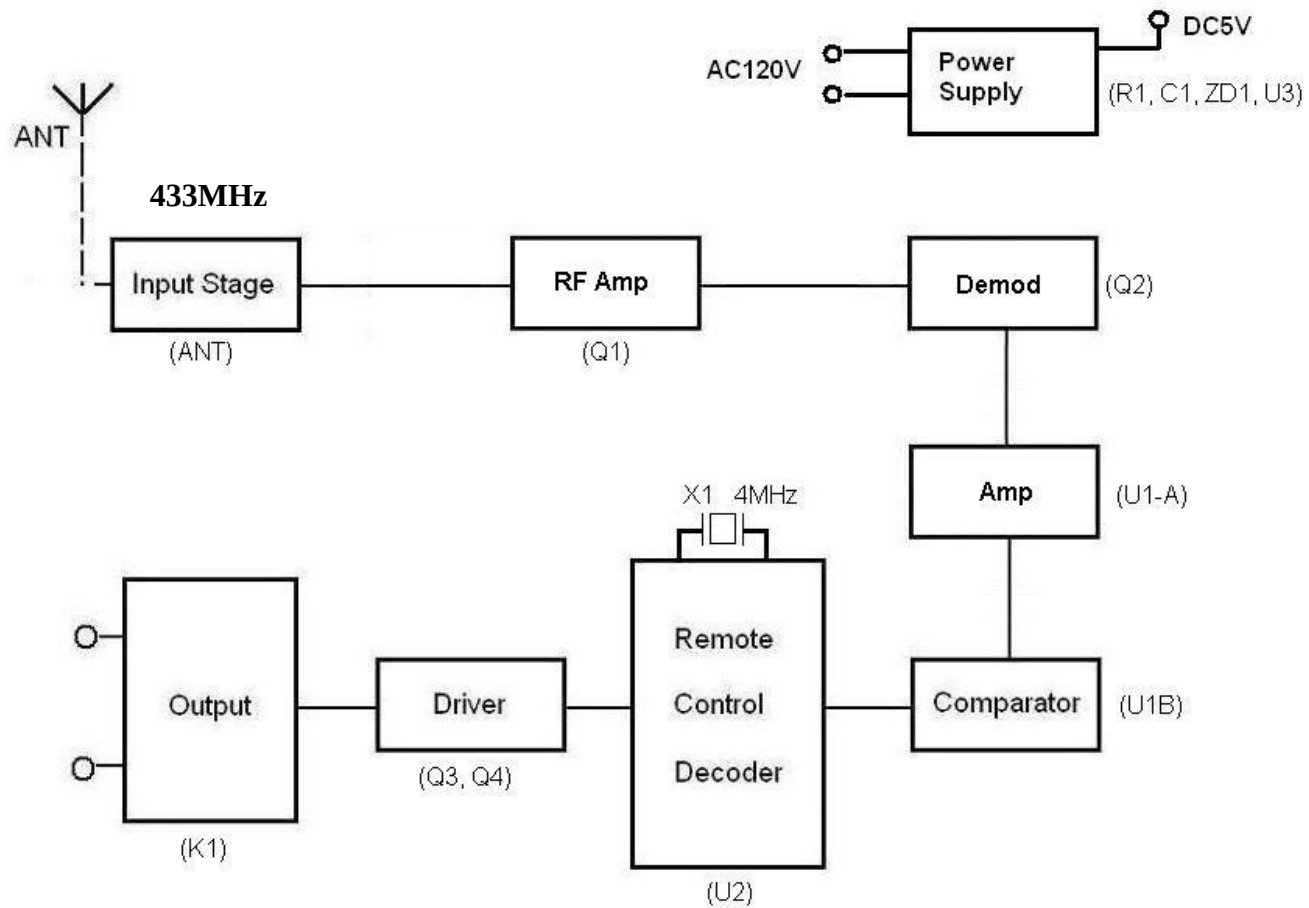
RF Switch - Operational Block Diagram (Receiver)
