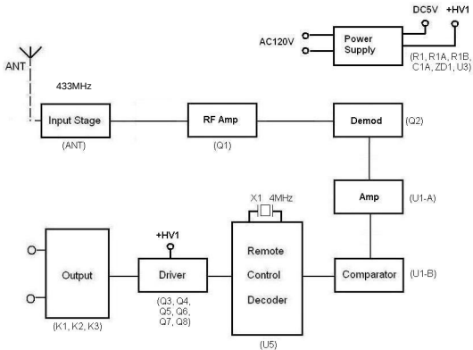
3-Stage On/Off Remote - Operational Block Diagram (Receiver)
