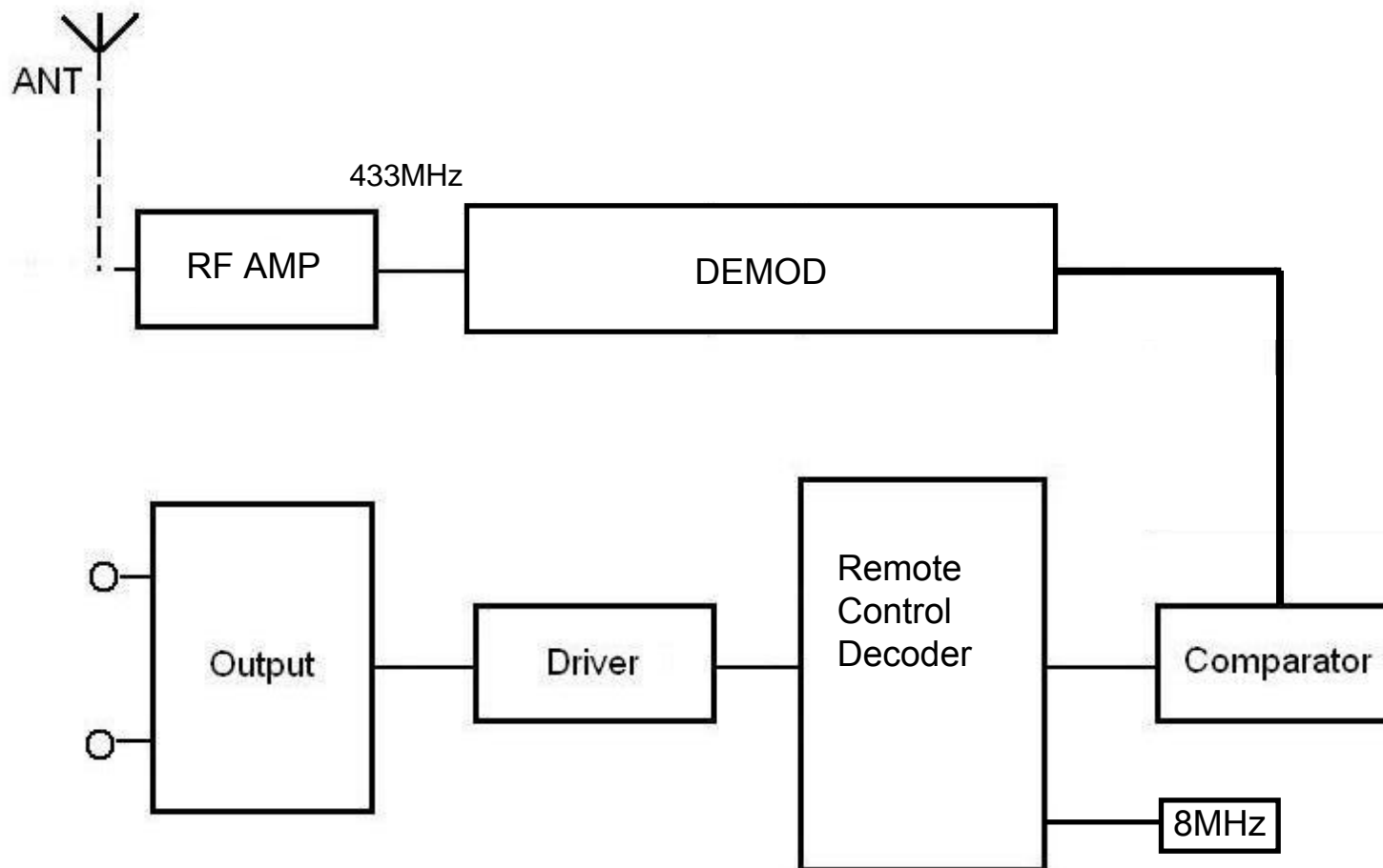
36 Inches Outdoor Fireplace - Operational Block Diagram (Receiver)
