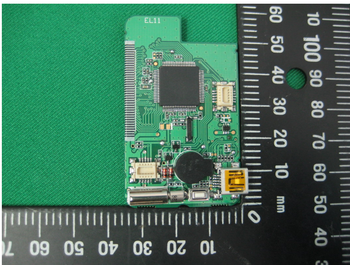
Rear View of Panel Board
