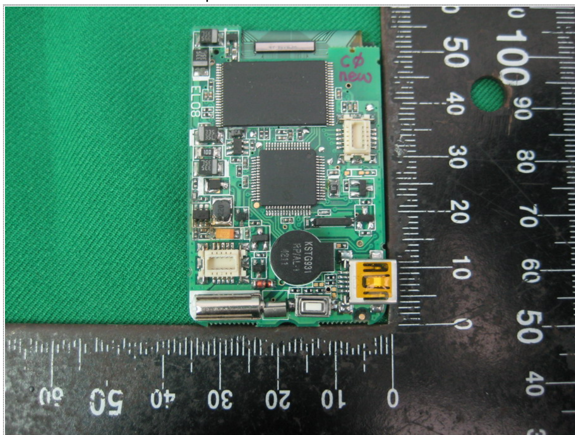
Solder View of Main Board-1
