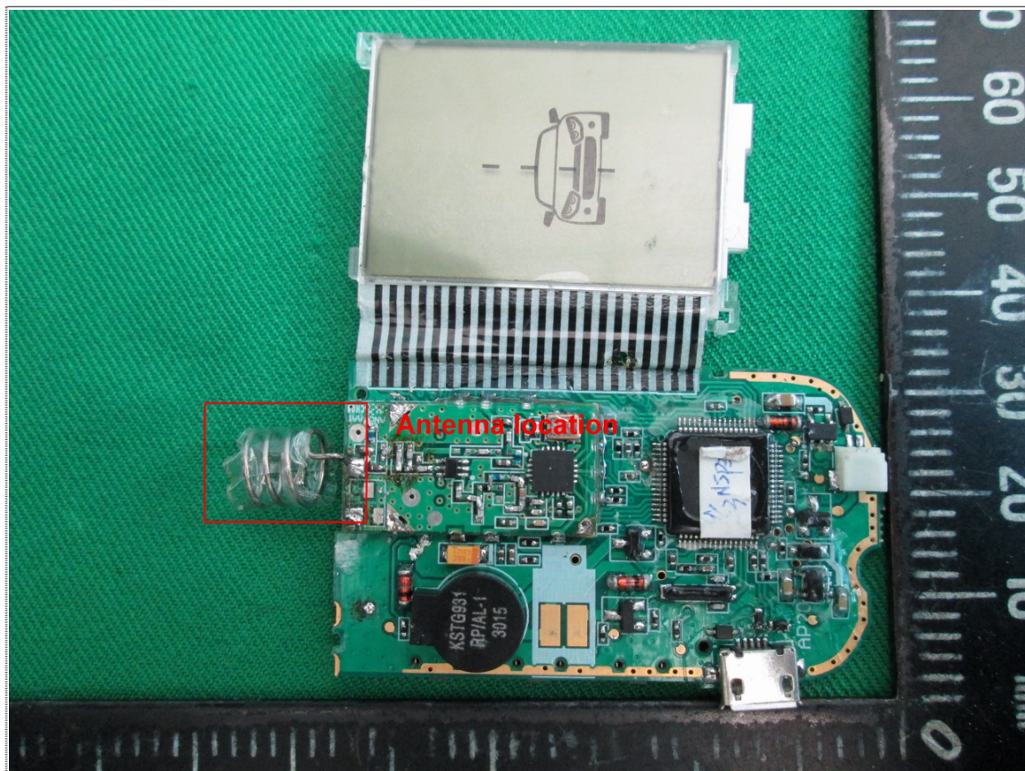
Antenna Location
