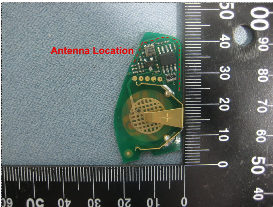
Antenna Location-1
