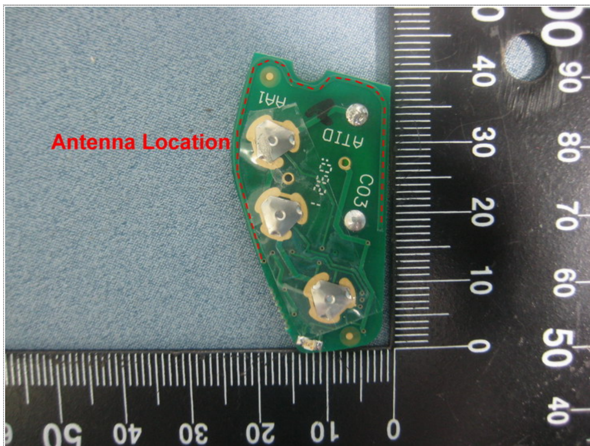
Antenna Location-2
