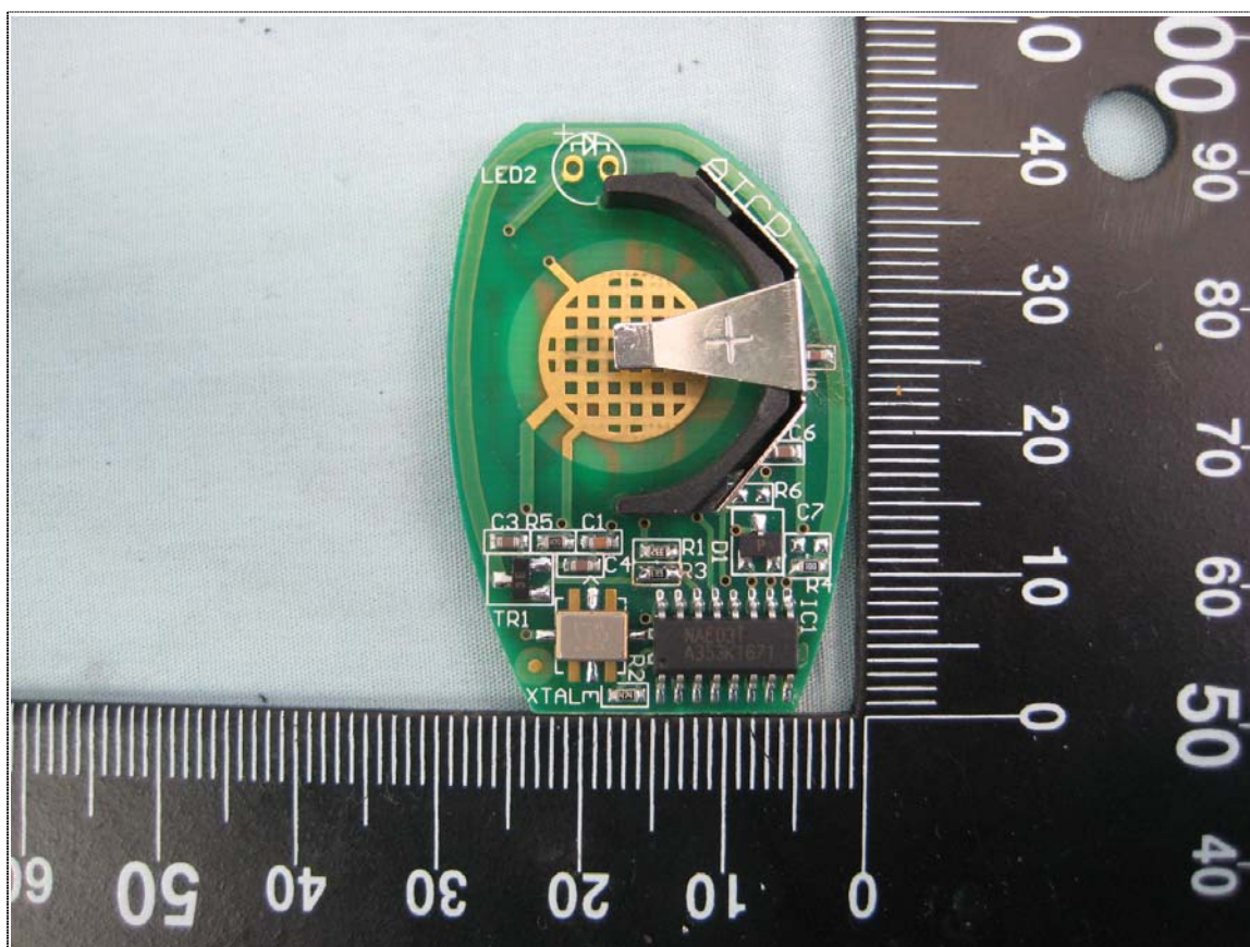
Component View of PCB Board (Model No.: PROTX5)
