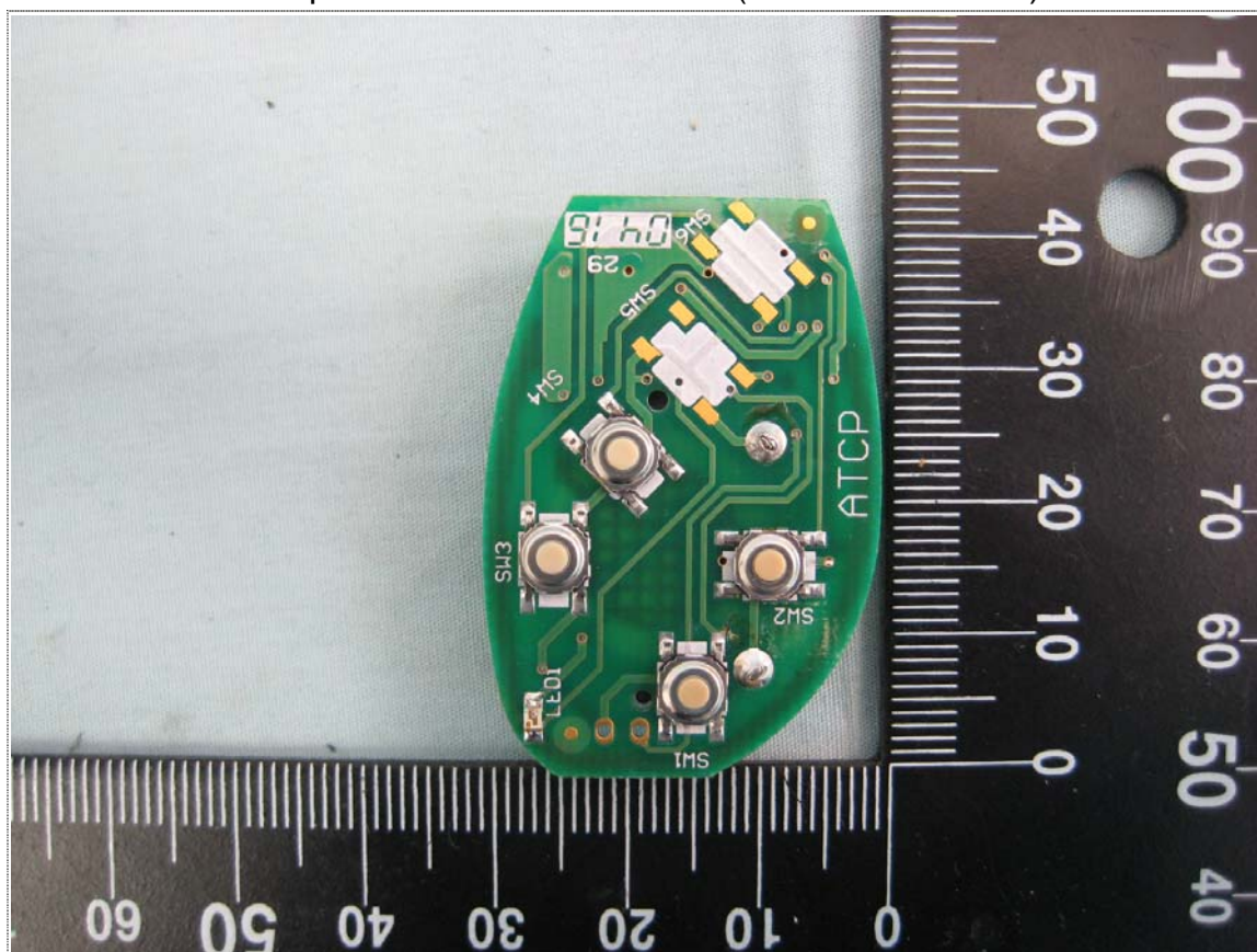
Solder View of PCB Board (Model No.: DIYTX)
