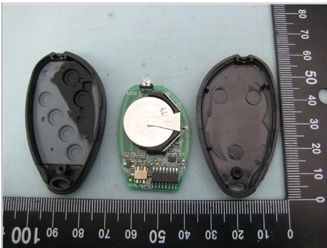
Inner View of EUT (Model No.: PROTX6)
