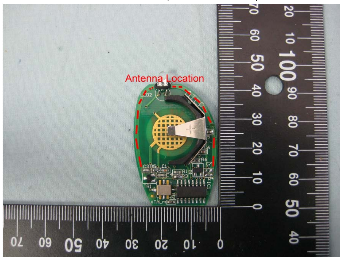
Antenna Location (Model No.: PROTX6)
