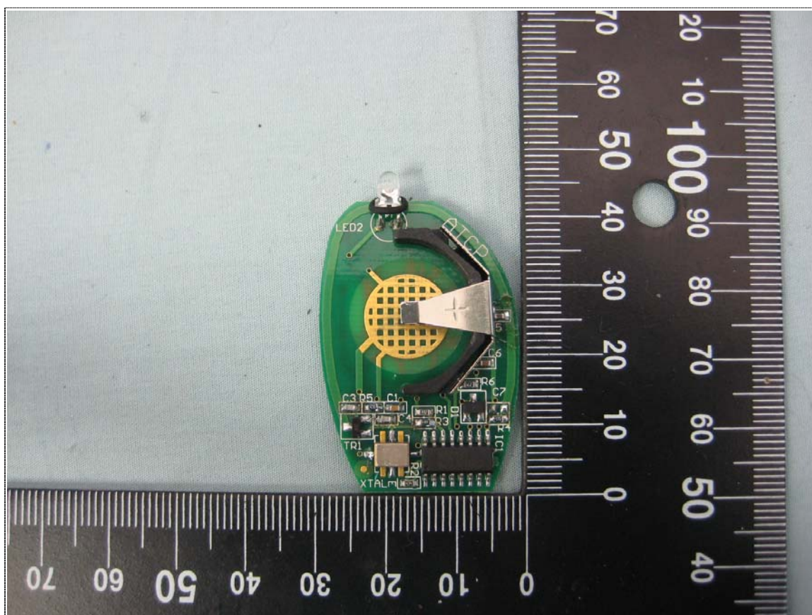
Component View of PCB Board (Model No.: PROTX6)
