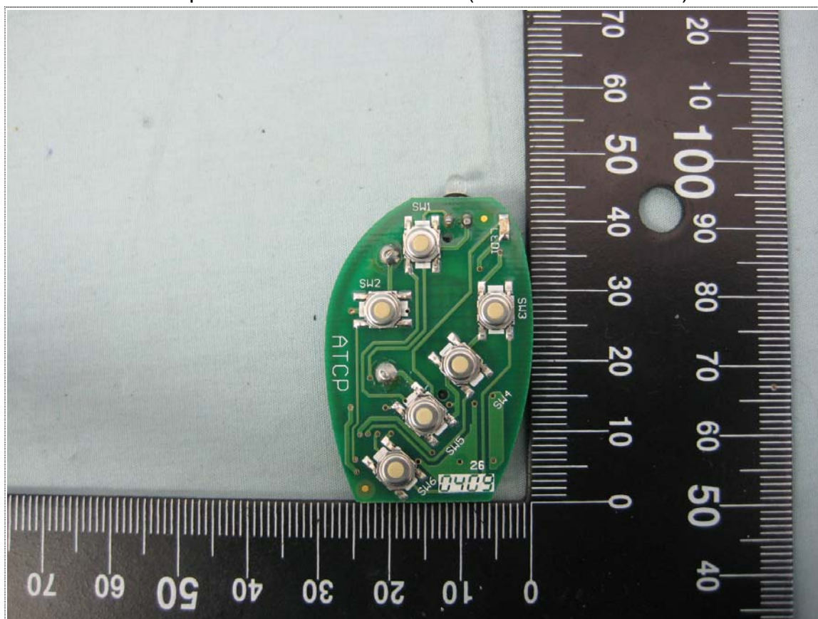
Solder View of PCB Board (Model No.: PROTX6)
