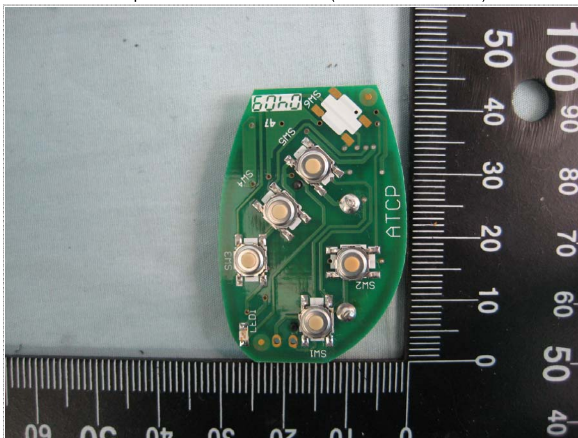
Solder View of PCB Board (Model No.: PROTX5)
