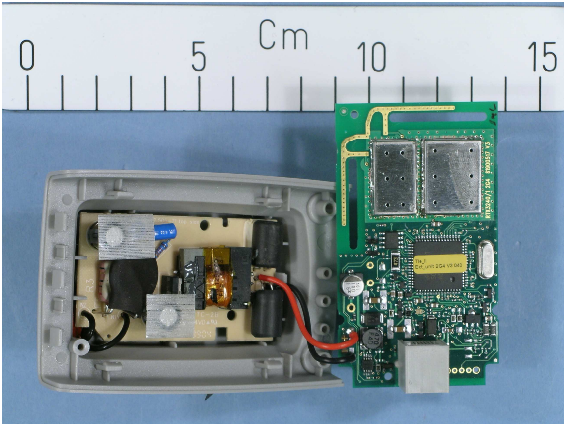
EXT 3240, View 1
