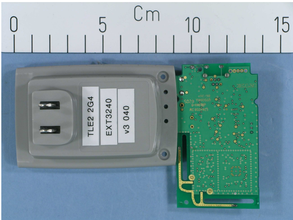
EXT 3240, View 2
