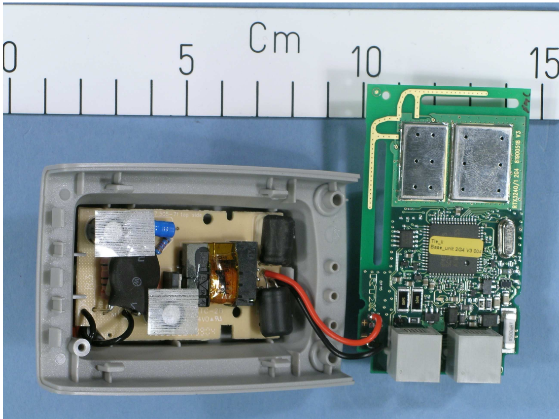
BS 3240, View 1
