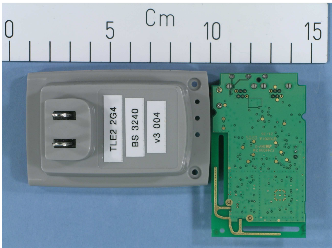
BS 3240, View 2
