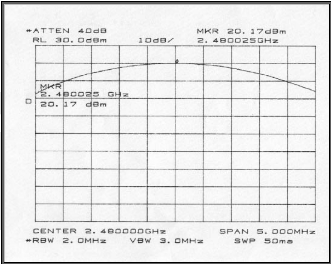
Power Out Channel 79
