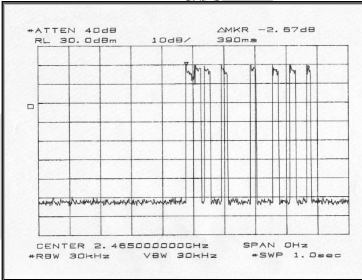
Channel Occupancy
