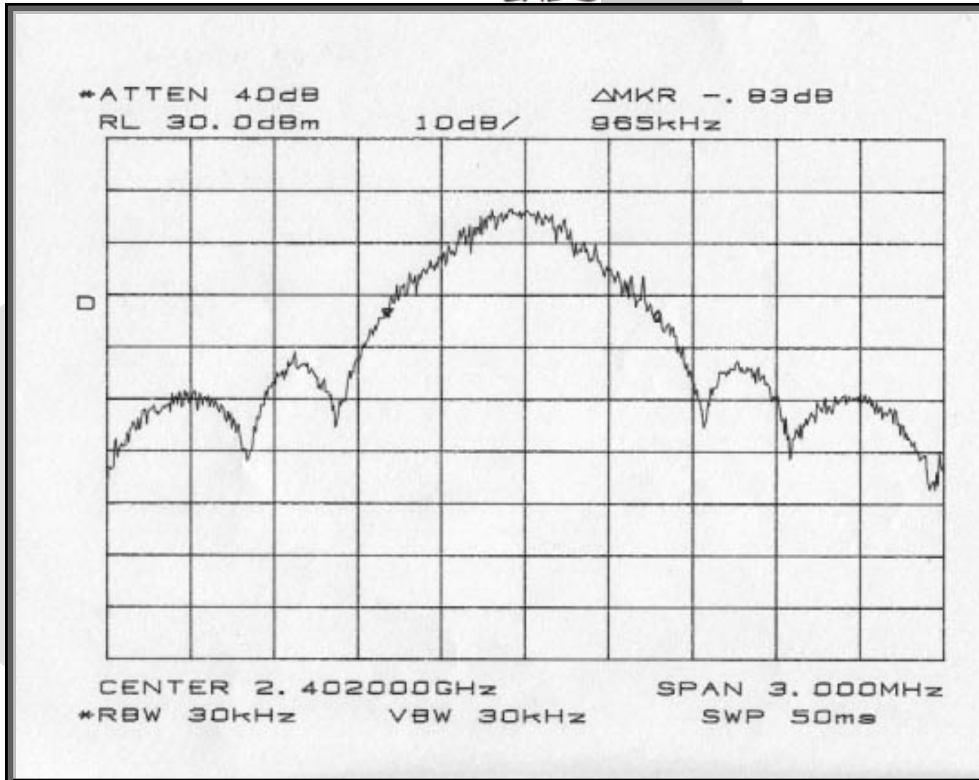
20dB Band Width Channel 1
