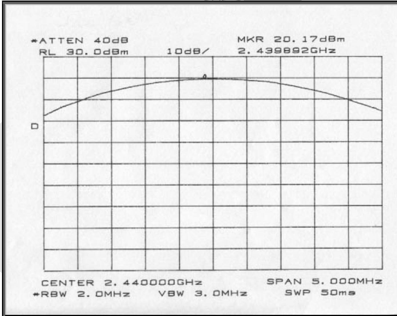
Power Out Channel 39
