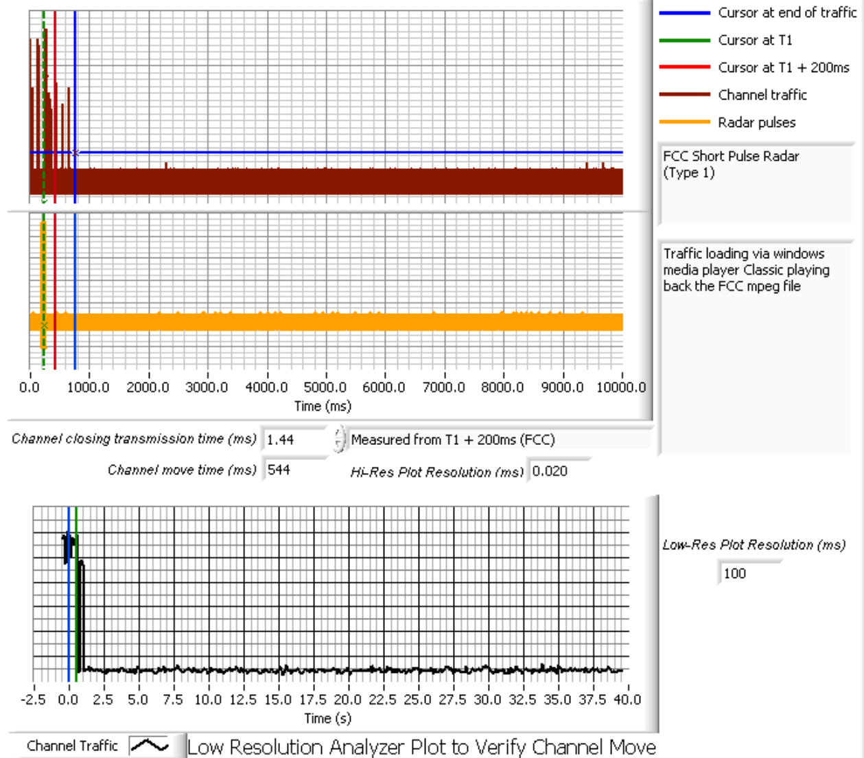
Figure 2: Channel Closing
