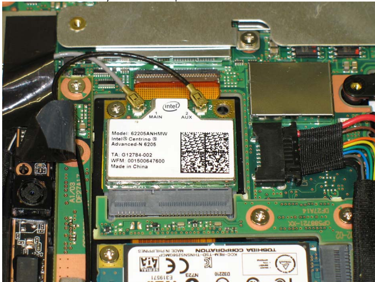
62205ANHMMW inside the Fujitsu TABLET Computer
