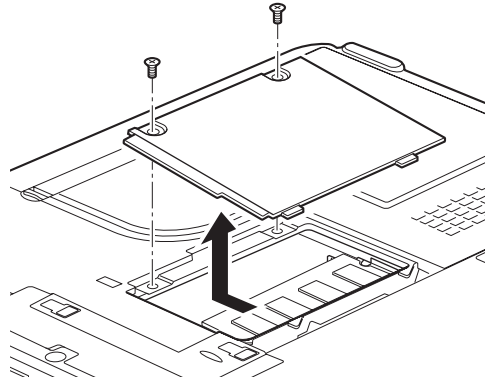
Figure 37. Opening Memory Compartment
