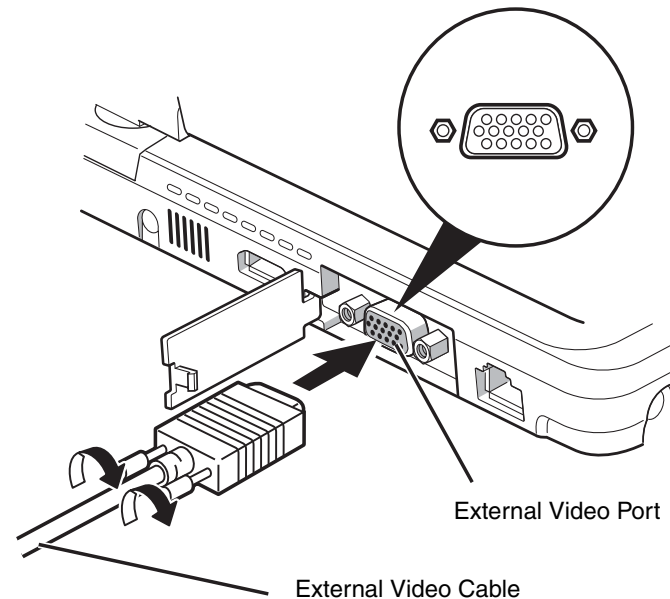
Figure 46. Connecting an External Video Device
