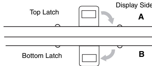
Figure 9. Latching/unlatching
