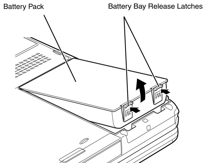
Figure 34. Removing a Battery
