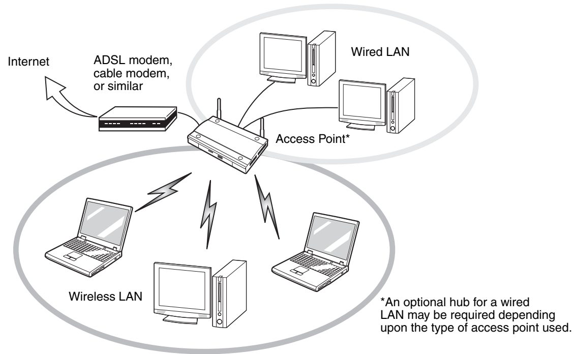
Figure 49. Access Point (Infrastructure) Mode Network
