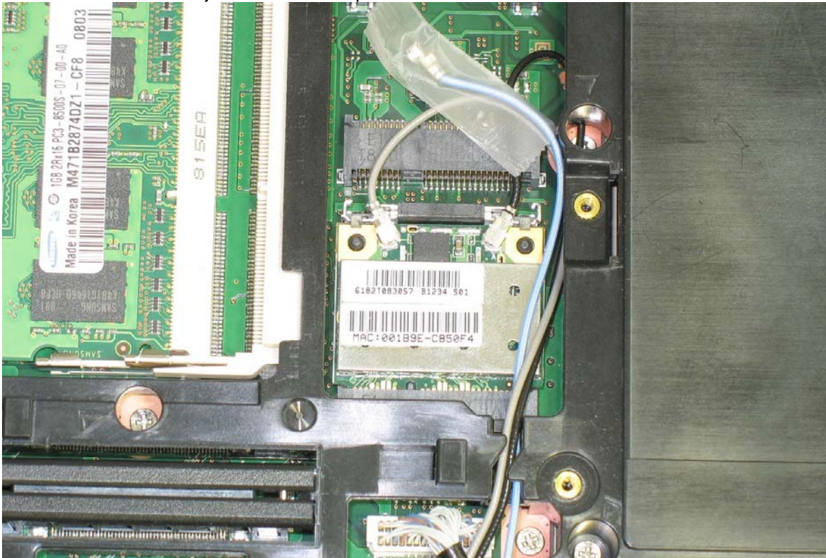
AR5BHB92 inside the Fujitsu TABLET Computer
