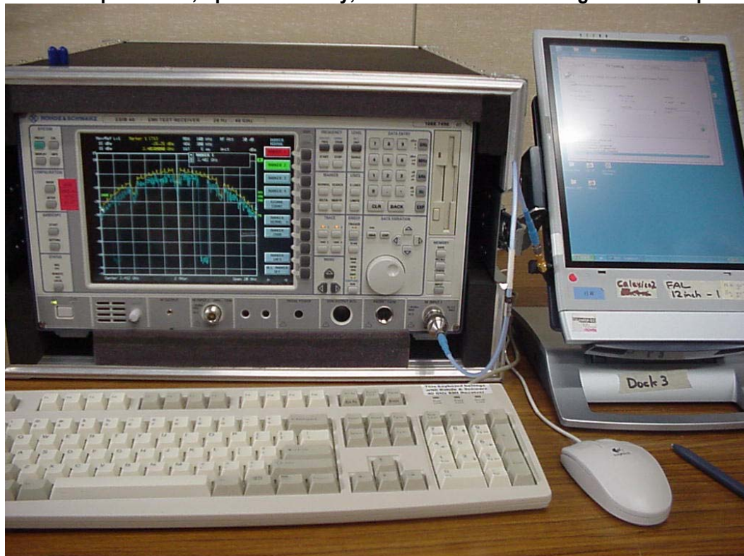
Peak Output Power, Spectral Density, Bandwidth and Band Edge Test Set Up.
