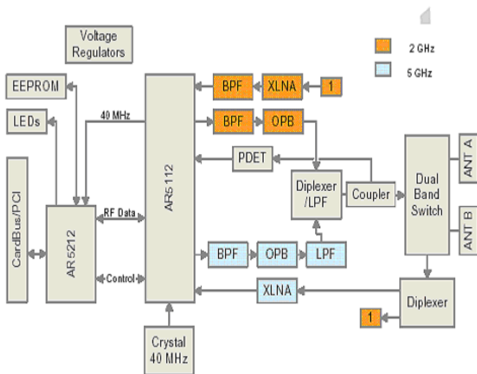
Figure WLL4030 Block diagram
