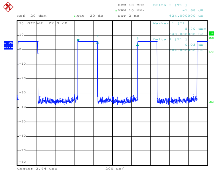
Bluetooth – LE 2Mbps
