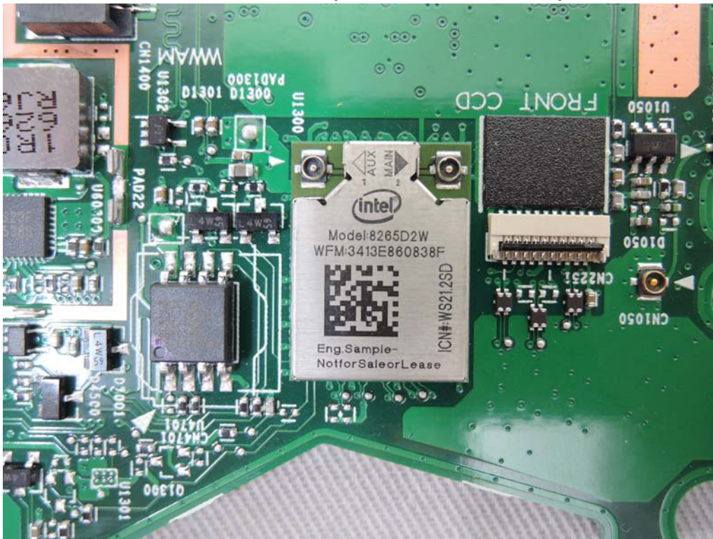
BT / WLAN Module (Model No.: 8265D2W) - 1
