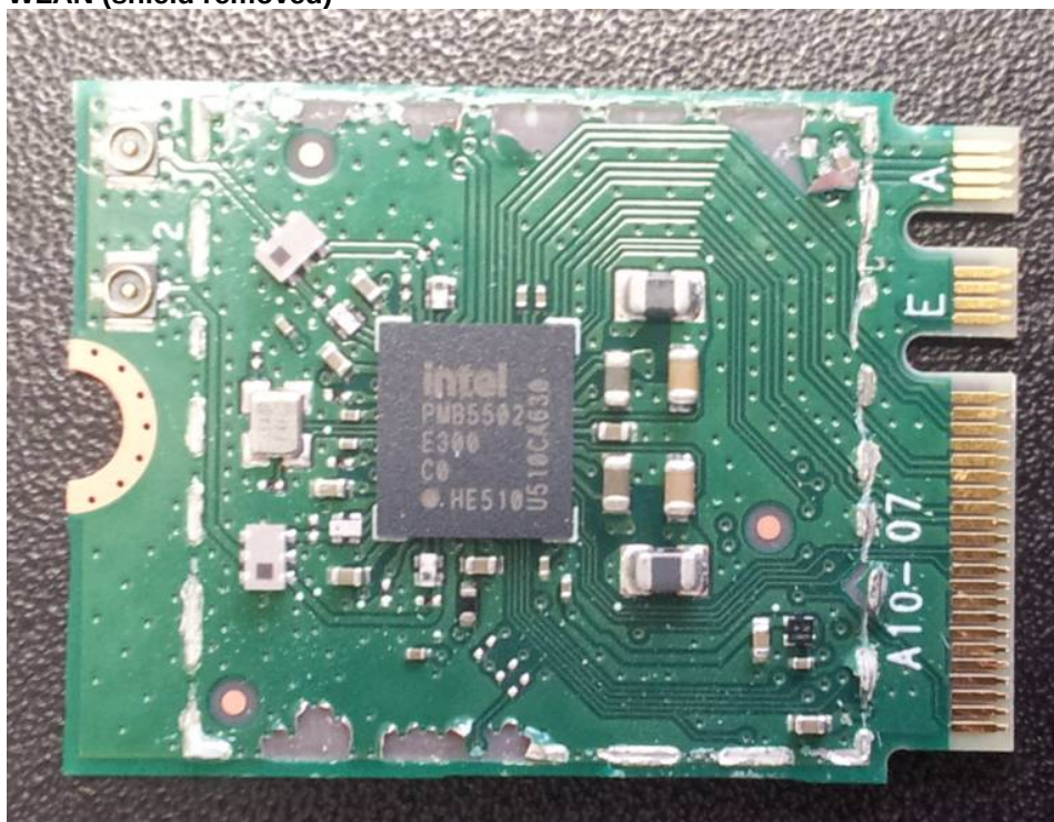
WLAN (shield removed)
