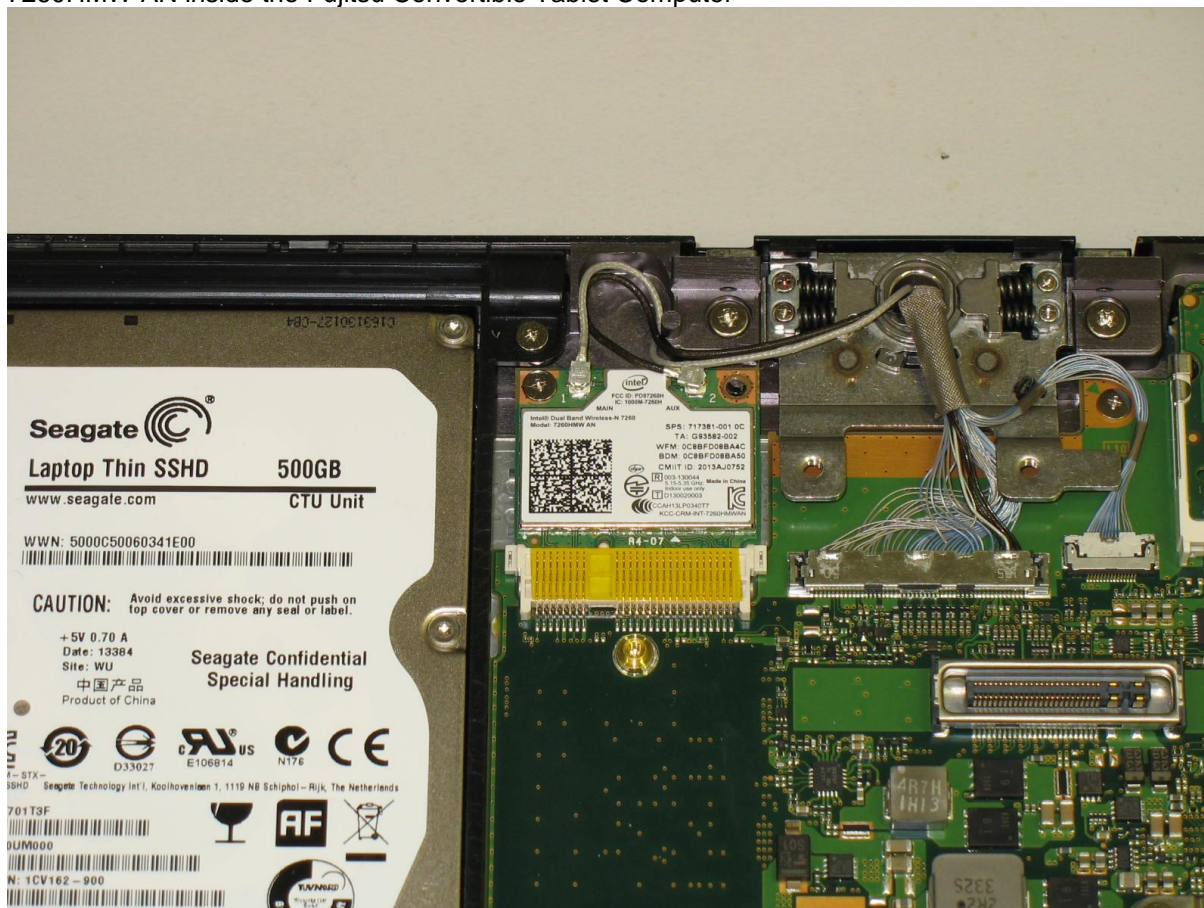
7260HMW AN inside the Fujitsu Convertible Tablet Computer
