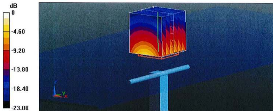
0 dB = 17.1 W/kg = 12.33 dBW/kg
