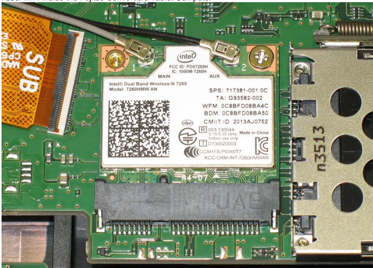
7260HMW inside the Fujitsu Convertible Tablet Computer
