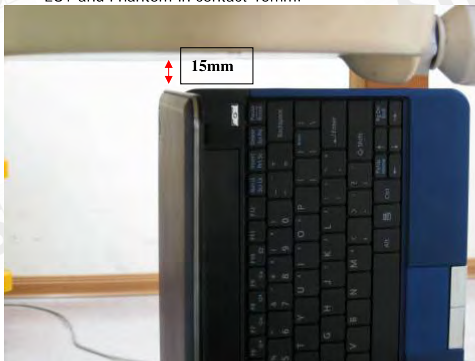
Fig.6 Right side of EUT is paralleled with flat phantom, and spacing between EUT and Phantom-in contact 15mm.
