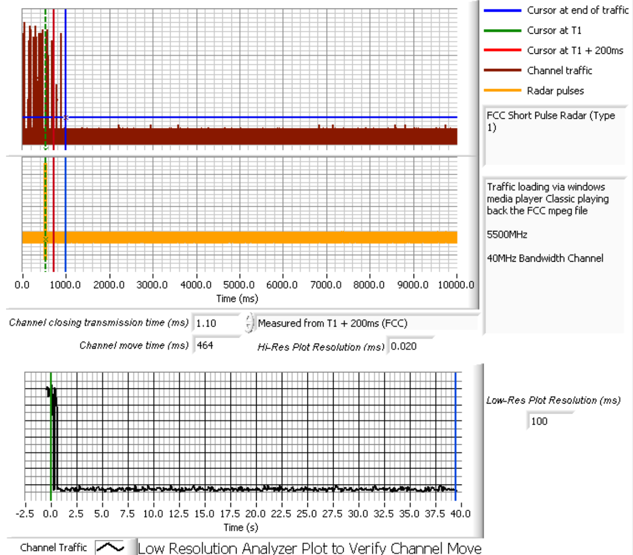
Figure 4 Channel Closing Time and Channel Move Time – 40 second plot, 40MHz BW
