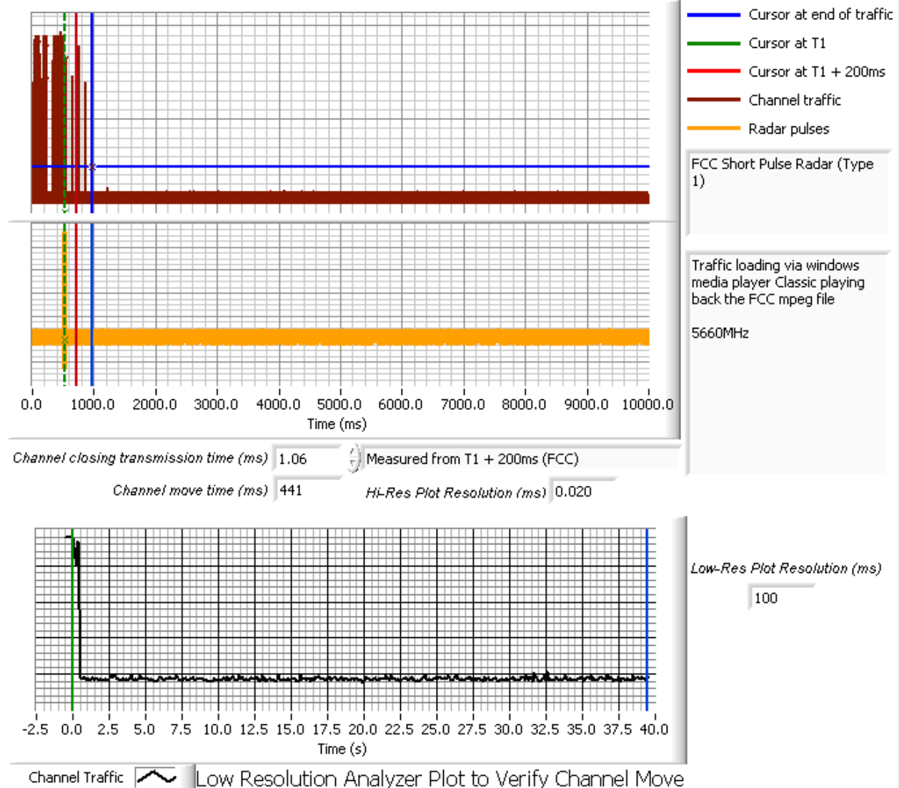
Figure 2 Channel Closing Time and Channel Move Time – 40 second plot, 20MHz BW
