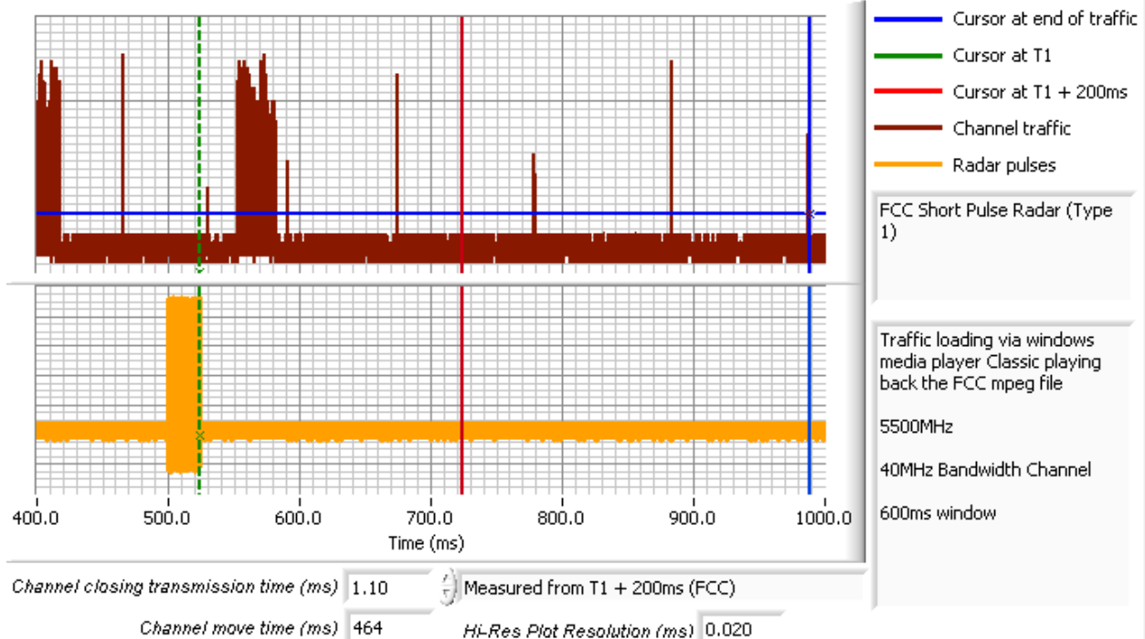
Figure 5 Close-Up of Transmissions Occurring More Than 200ms After The End of Radar, 40MHz BW
