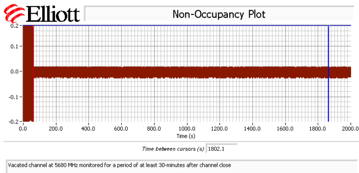
Figure 6 Radar Channel Non-Occupancy Plot (Associated Test)
