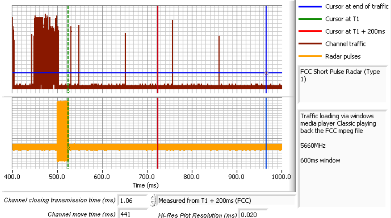
Figure 3 Close-Up of Transmissions Occurring More Than 200ms After The End of Radar, 20MHz BW
