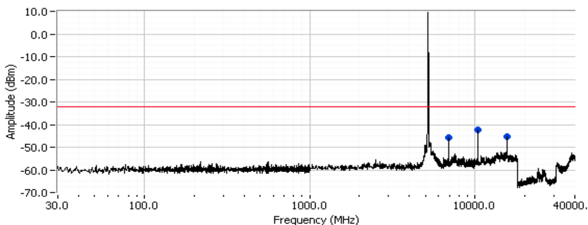
Out of Band Spurious Emissions - Antenna Conducted at 5200 MHz (legacy mode)
