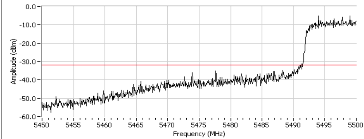
Out Of Band Spurious Emissions at 5510 MHz, n40 Mode, Bandedge at 5460 MHz
