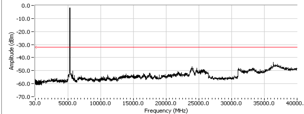
Out Of Band Spurious Emissions at 5510 MHz, n40 Mode, Bandedge at 5460 MHz
