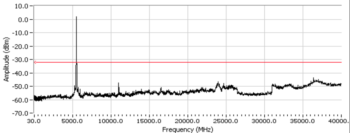
Out Of Band Spurious Emissions at 5510 MHz, n40 Mode
