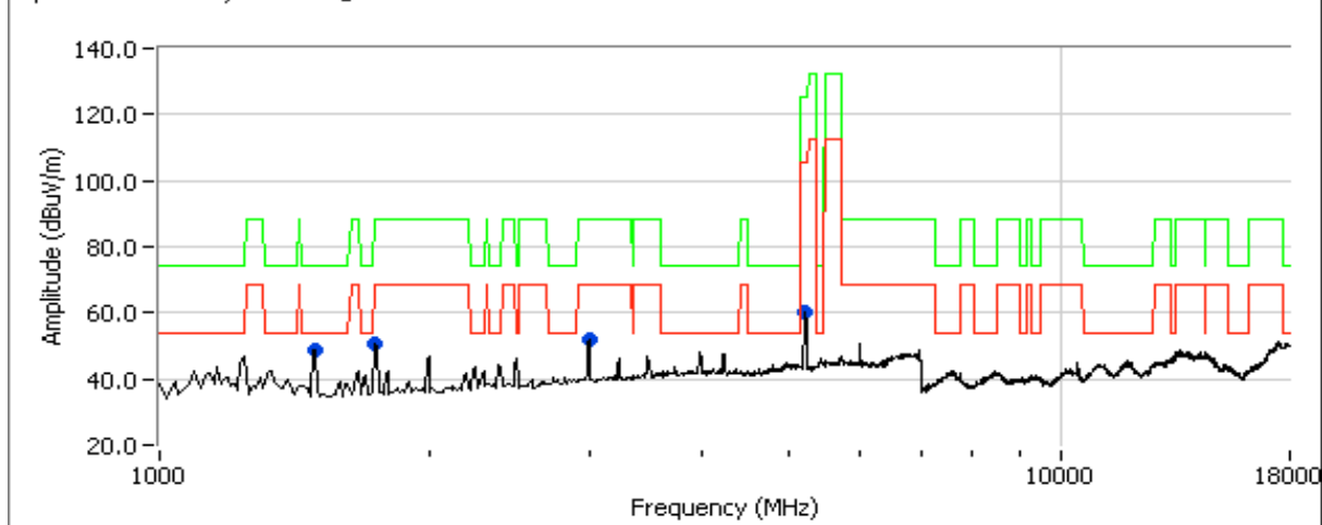
Spurious Emissions, Channel @ 5270MHz mode n40
