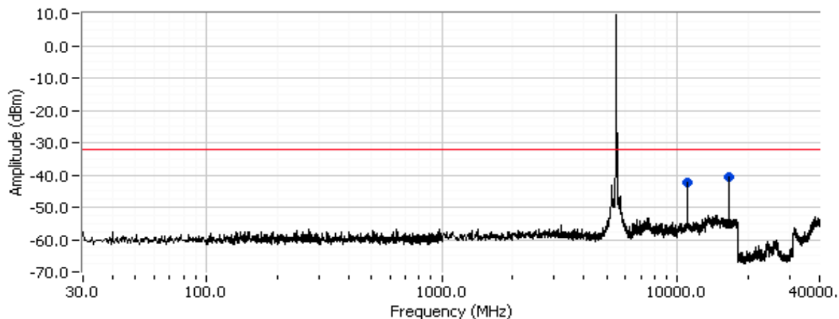
Out Of Band Spurious Emissions at 5500 MHz, Bandedge at 5460 MHz
