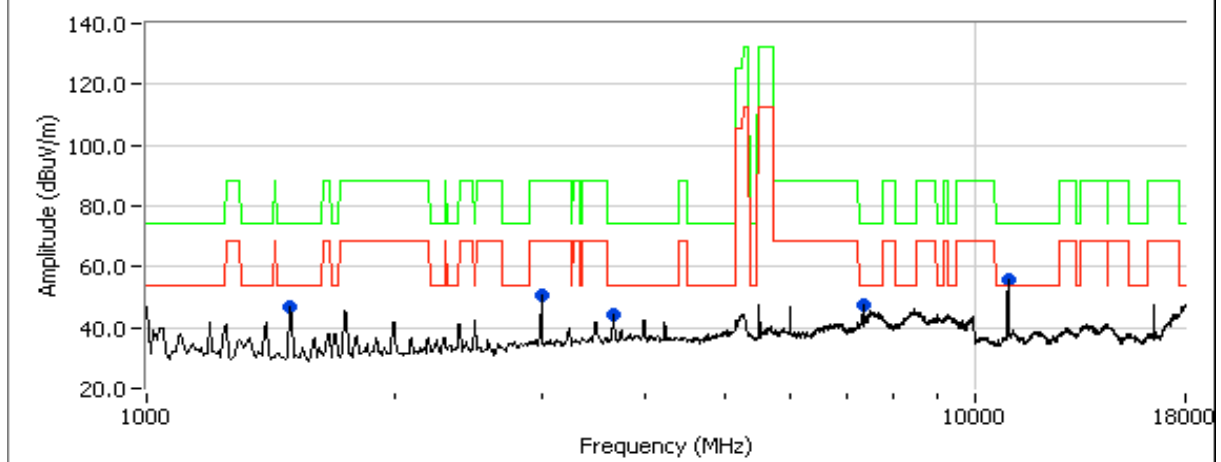
Spurious Emissions, Channel @ 5500 MHz Mode a
