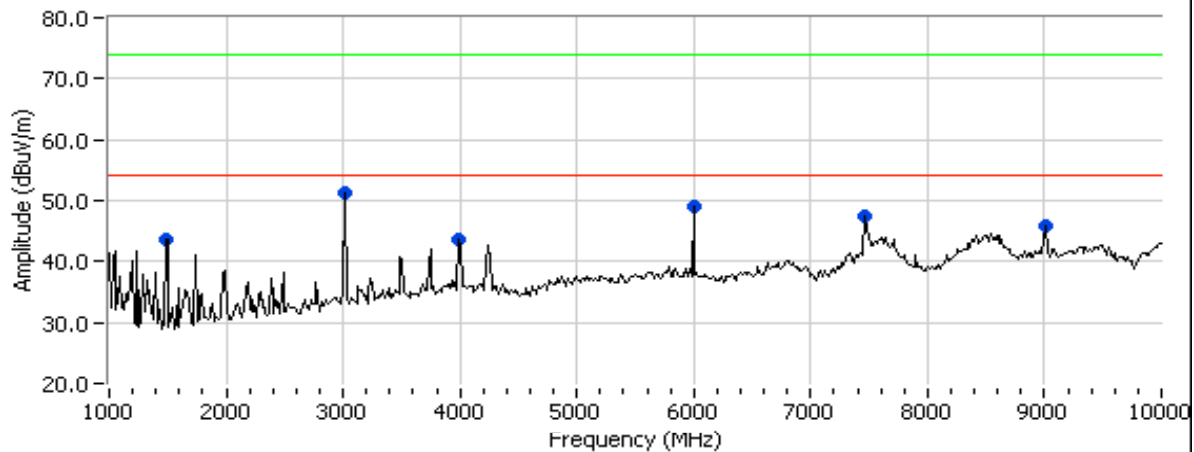
Chain B RX Channel @ 5600 MHz
