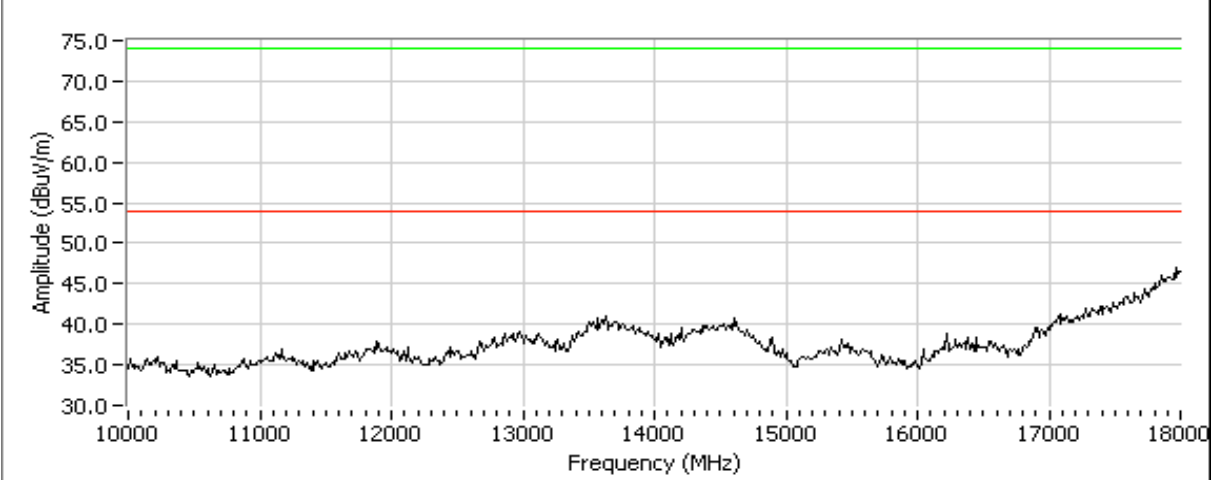
Chain A RX Channel @ 5280 MHz
