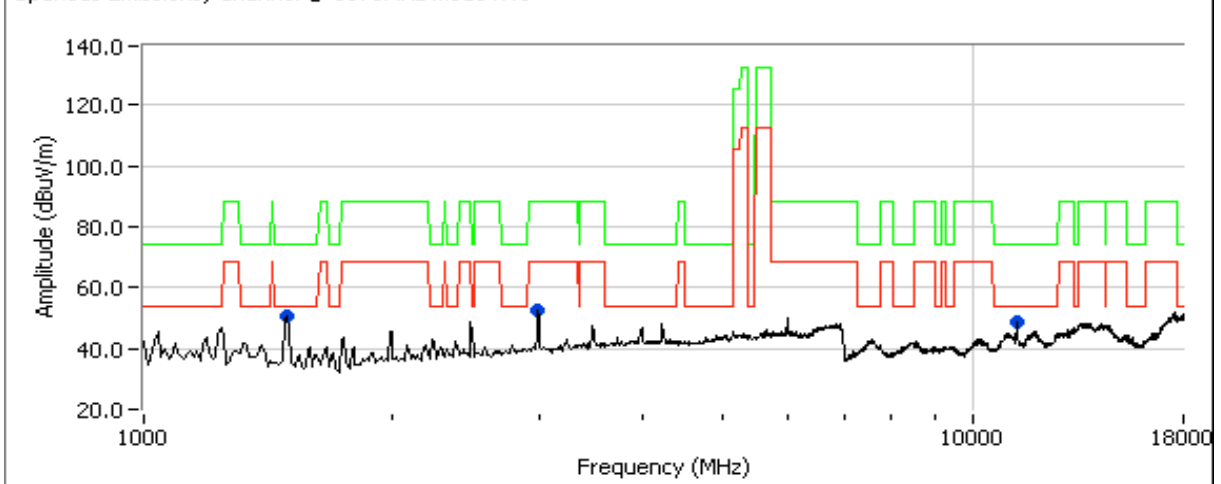
Spurious Emissions, Channel @ 5670MHz mode n40
