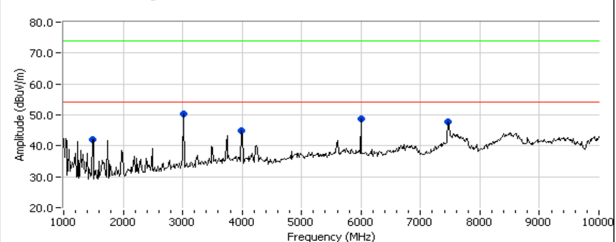
Chain A RX Channel @ 5600 MHz
