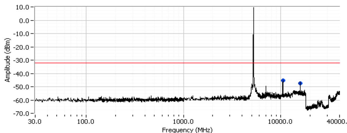
Out of Band Spurious Emissions - Antenna Conducted at 5240 MHz (legacy mode)
