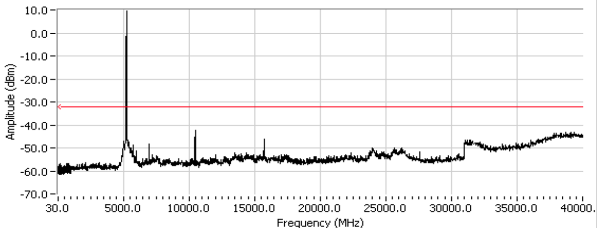
Out of Band Spurious Emissions at 5240 MHz, n20 Mode
