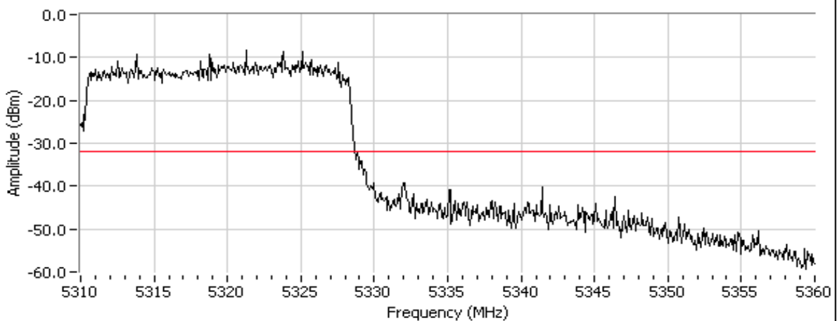
Out Of Band Spurious Emissions at 5310 MHz, n40 Mode, Bandedge at 5350 MHz
