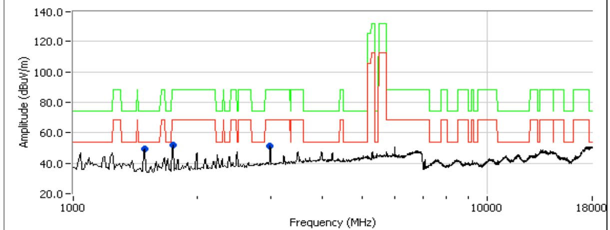
Spurious Emissions, Channel @ 5310MHz mode n40
