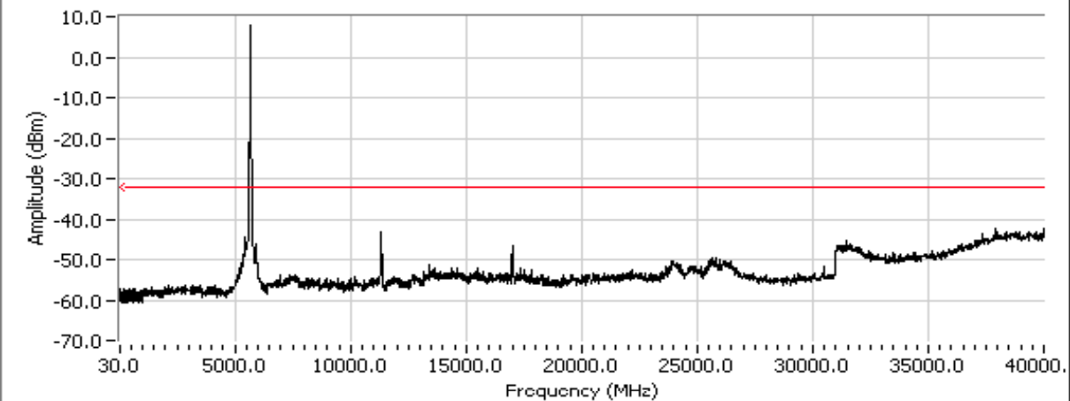
Out Of Band Spurious Emissions at 5670 MHz, n40 Mode
