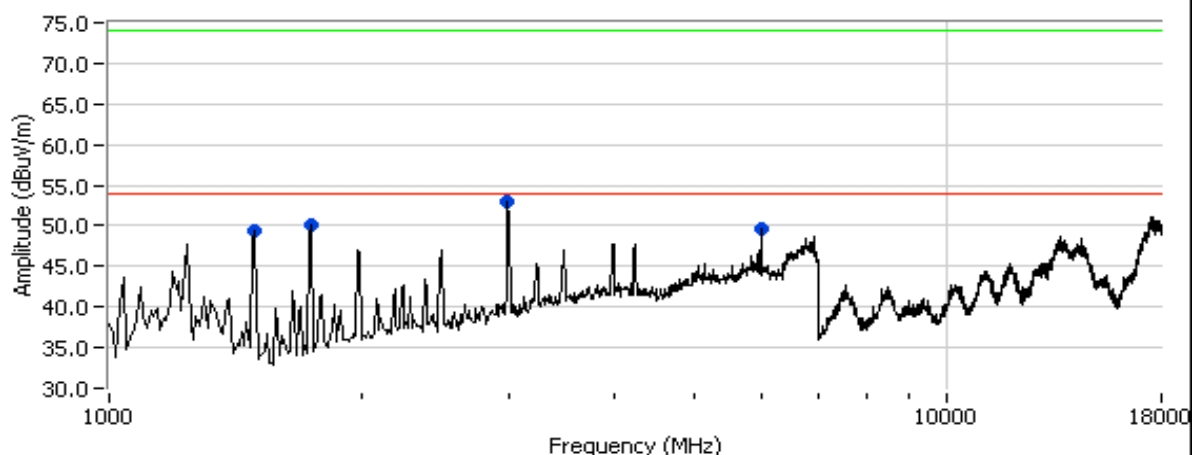
Channel @ 5200MHz
