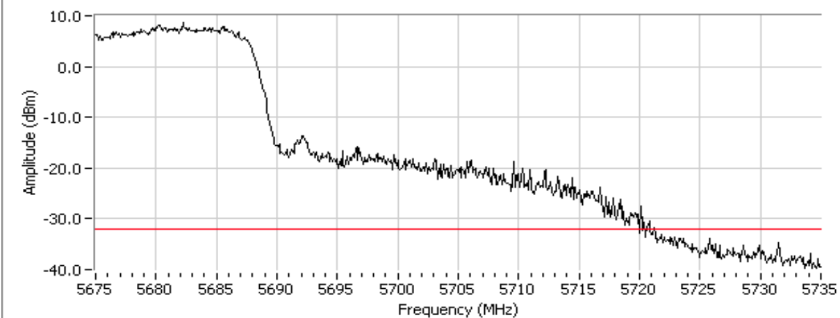
Out Of Band Spurious Emissions at 5670 MHz, n40 Mode, Bandedge
